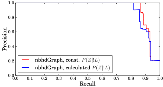
Figure 10: Precision-recall results on the KITTI 05 sequence, comparing the results using a constant value for P(\mathcal{Z}_q|\bar{\mathcal{L}}_i) , and one which calculated P(\mathcal{Z}_q|\bar{\mathcal{L}}_i) using the dataset ground-truth.
