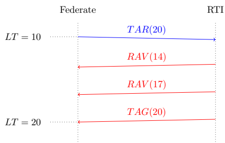
Fig. 2. Typical execution sequence.
