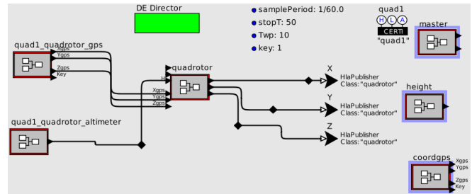
Fig. 4. A Ptolemy Actor modeling a control-law connected to the external world through HLA
