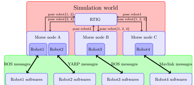
Fig. 7. A Morse multinode instantiation with four robots on three different nodes. Each robot software layer interacts with Morse using its specific middleware. The red area denotes the simulation world, where data are exchanged through HLA. The green area denotes the interaction between the simulation and real software to be tested.
