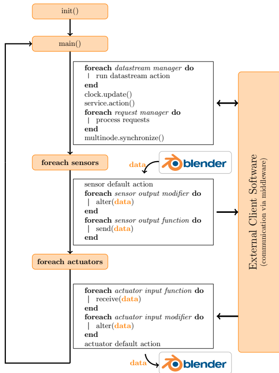
Fig. 1. Morse main loop overview
