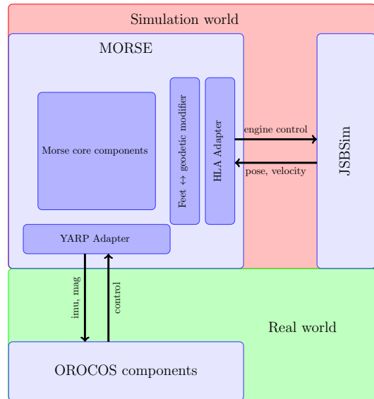
Fig. 6. An OrocOS-based robot simulation with Morse and JSBSim. The red area denotes the simulation world, where data are exchanged through HLA. The green area denotes the interaction between the simulation and real software to be tested, using a robotic middleware (here YARP).
