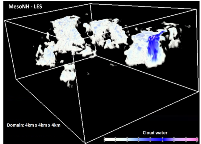
Fig. 6 Meso-NH LES simulation: liquid cloud water content of the cumulus formed at 1h30 PM (ARM Southern Great Plains, June 21, 1997 conditions)
