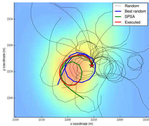
Fig. 3 Illustration of the trajectory generation process in a realistic wind field, for a planning horizon \Delta T = 20 seconds. Projections on the xy plane for the random sampling initialization, optimized trajectory and final trajectory executed by the UAV are shown. The red star represents the initial position and the map colors shows the vertical component of the wind – with no particular units, the redder being the highest.
