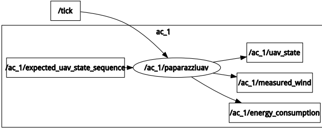
Fig. 8: ROS graph of paparazziuav
