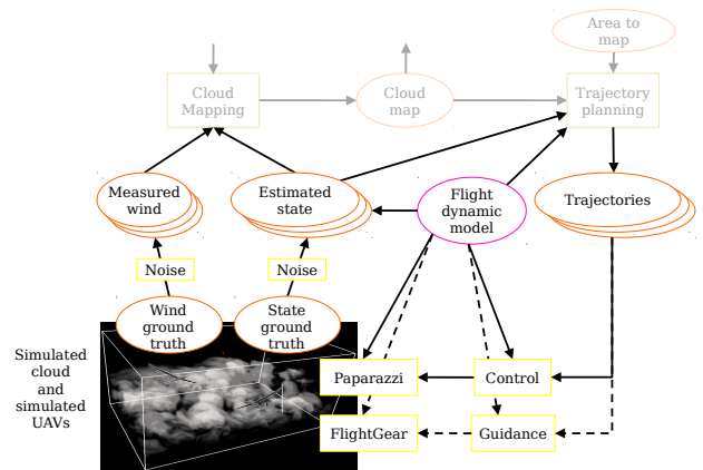
Fig. 3: Schematic view of the architecture of the simulated system. The figure focuses on the simulated processes. The same processes of figure 2 are integrated in the overall simulation, and a second option to control the UAVs using a guidance scheme to follow the trajectories has been added (dashed arrows with the Guidance process).
