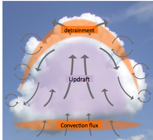
Fig. 1: Schematic representation of a cumulus cloud. The arrows represent wind velocities, the orange blobs denote areas where mixing is occurring between the cloud and the surrounding atmosphere. This representation is very coarse: for instance the updrafts in the center of the cloud are known to behave as “bubbles” when the cloud is young. The cloud dimensions can vary from one to several hundreds of meters. Such a conceptual model encodes various laws, e.g. that relate the cloud dimensions to the inner wind speeds.
