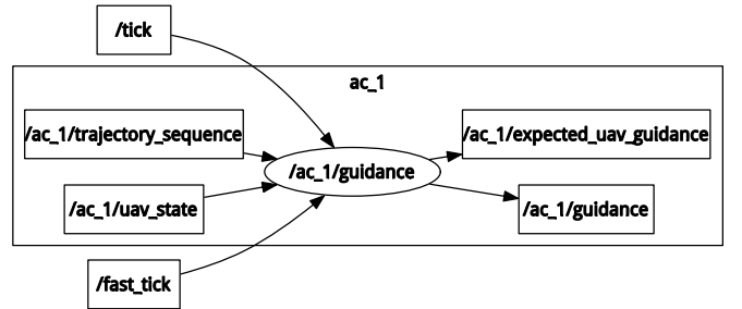
Fig. 13: guidance node ROS graph
