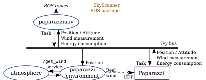
Fig. 7: Interface scheme between Paparazzi and SkyScanner ROS package
