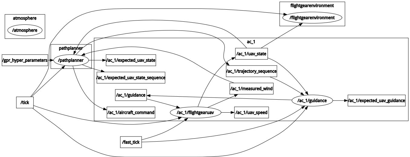
Fig. 15: ROS graph of the complete FlightGear execution loop.
