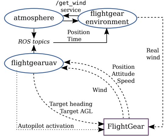
Fig. 9: Interface scheme between FlightGear and SkyScanner ROS package
