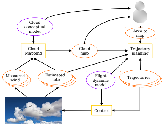
Fig. 2: Overall architecture of the fleet control. Orange, yellow and purple boxes respectively denote information, processes and models. Given a coarse conceptual model of the cloud and the map built by the UAVs so far, the user tasks the fleet with an area to explore. The trajectory planner exploits the cloud map to find the trajectories that optimize the information gathering and the energy expenses, which are sent to the UAVs. Note the importance of the Flight Dynamic Model of the UAVs, which is used by three different processes.
