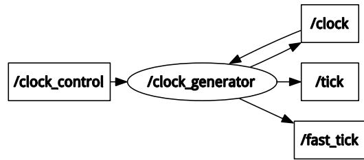
Fig. 5: Clock generator ROS graph
