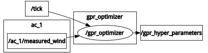
Fig. 12: GP optimizer ROS graph
