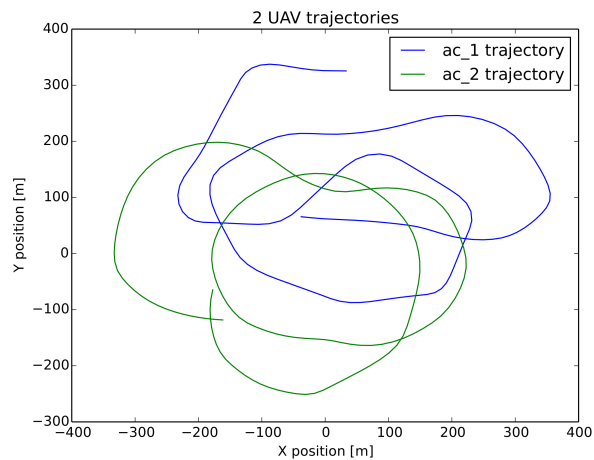
Fig. 16: Trajectories resulting from the simulation of the exploration of a cloud by two UAVs
