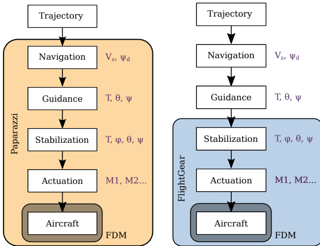
Fig. 4: Two different options to simulate the UAVs. Left, Paparazzi solution, where the full control stack is available and trajectories are tracked using a carrot chasing approach. Right, FlightGear solution: the guidance stage of the control stack must be ensured by an external process to track trajectories.
