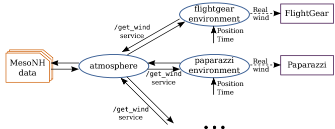
Fig. 6: Interface between MesoNH data (the cloud environment) and the two flight simulators
