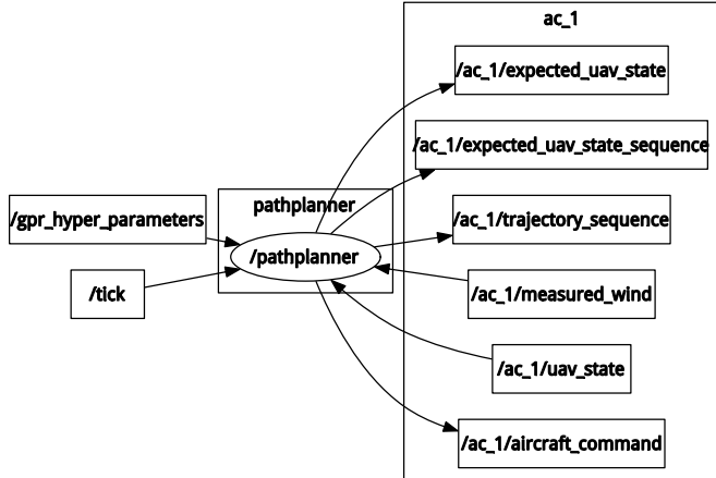
Fig. 11: Path planner ROS graph
