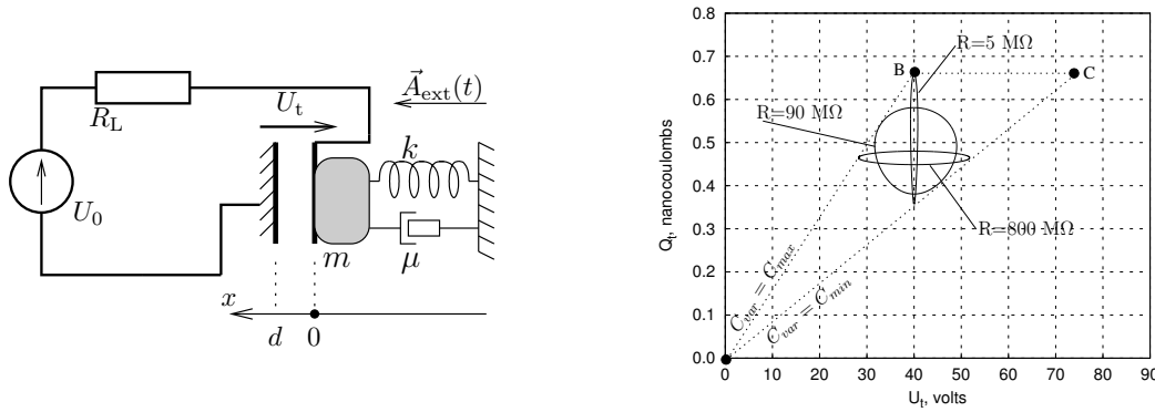
Figure 1. Schematic view of the continuous conditioning circuit (left) and charge-voltage diagrams for different values of load resistance at U_0=40\text{ V} (right). X=12\text{ }\mu\text{m} , f=150\text{ Hz} .
