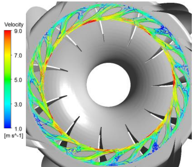
Fig. 22 Flow field inside the wicket gates.
