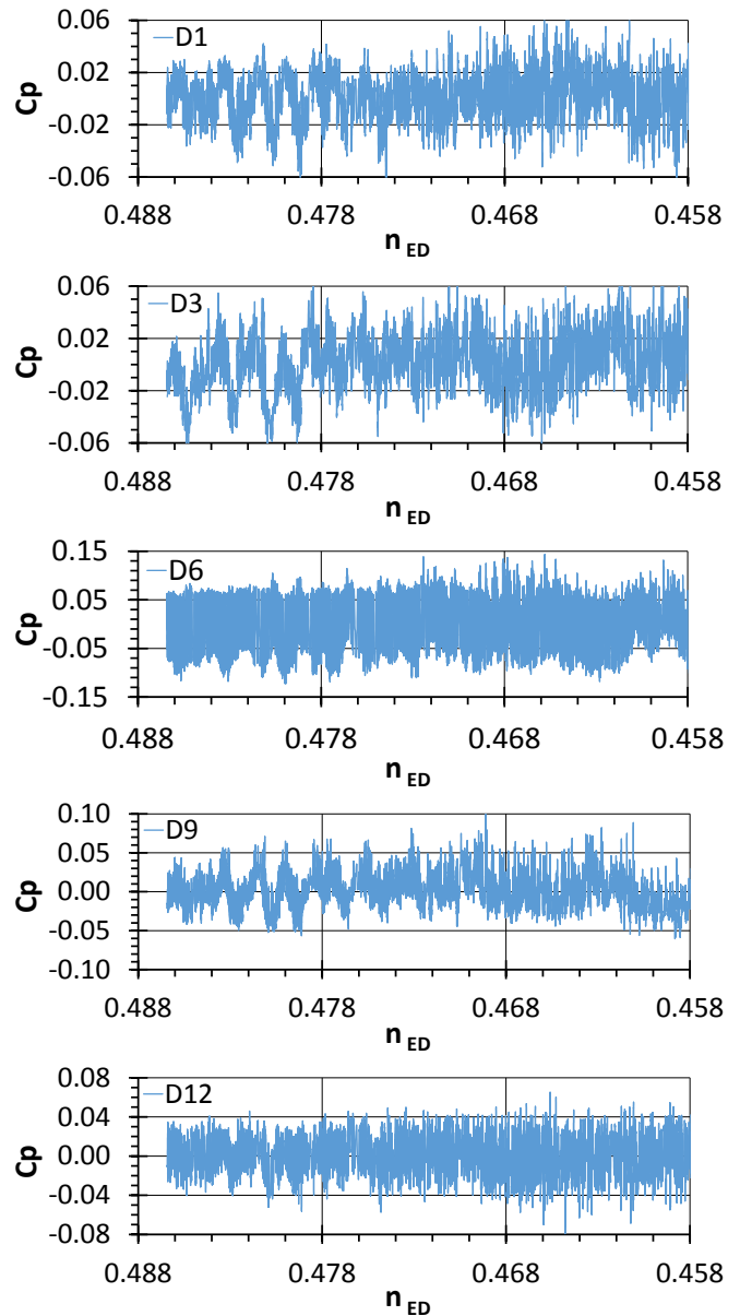
Fig. 12 Pressure coefficient versus speed factor acquired in the wicket gate.
