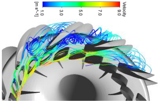
Fig. 9 Flow field inside the pump-turbine for n_{ED}=0.482 .
