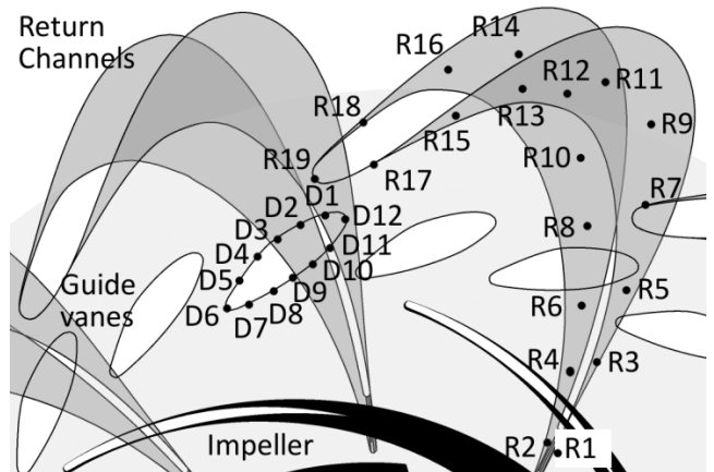
Fig. 2 Detail and sketch of the tested configuration ( \lambda=8^\circ ) with the distribution of monitor points.
