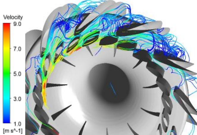
Fig. 21 Flow field inside the pump-turbine at different speed factor.
