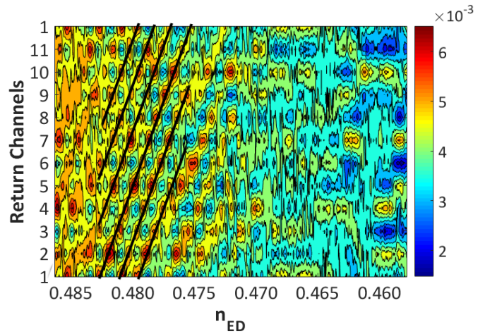
Fig. 8 Numerical dimensionless discharge-speed curves of the return channels.
