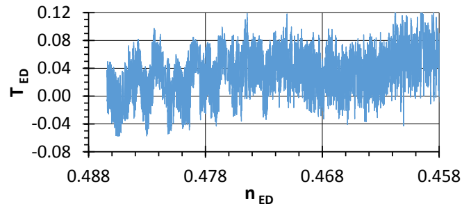
Fig. 13 Wicket gate torque factor versus speed factor.
