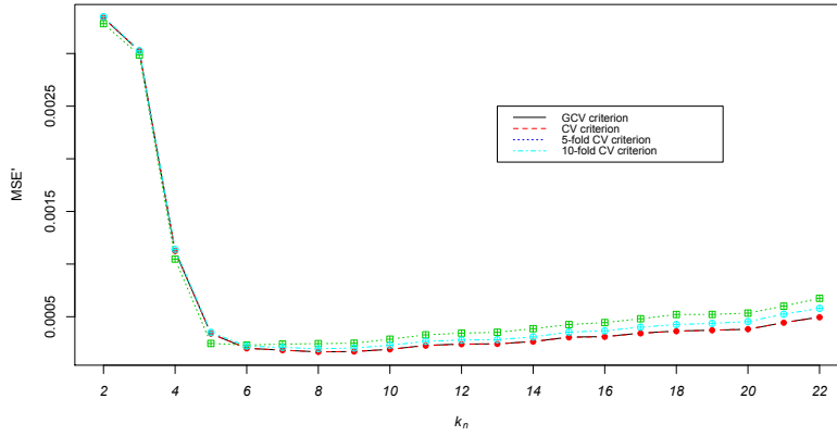
Fig. 2 GCV, CV and K-fold criteria for different values of dimension k_n : best dimension k_n^* = 8 and MSE' (\times 10^4) = 1.6640 (in GCV criterion case), best dimension k_n^* = 6 and MSE' (\times 10^4) = 2.3081 (in 5-fold CV criterion case), best dimension k_n^* = 8 and MSE' (\times 10^4) = 1.9584 (in 10-fold CV criterion case), best dimension k_n^* = 8 and MSE' (\times 10^4) = 1.6598 (in CV criterion case), for the model_1 .
