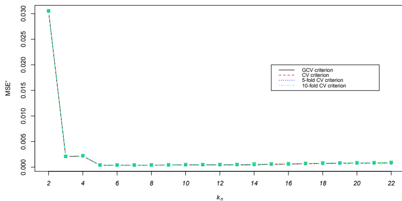
Fig. 3 GCV, CV and K-fold criteria for different values of dimension k_n : best dimension k_n^* = 5 and MSE' (\times 10^4) = 3.7589 (in GCV criterion case), best dimension k_n^* = 5 and MSE' (\times 10^4) = 4.2132 (in 5-fold CV criterion case), best dimension k_n^* = 5 and MSE' (\times 10^4) = 3.9758 (in 10-fold CV criterion case), best dimension k_n^* = 5 and MSE' (\times 10^4) = 3.7270 (in CV criterion case), for the model 2 .
