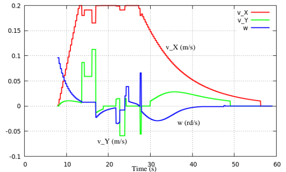
Fig. 6. MPO700 Control inputs
