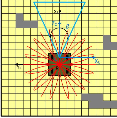
Fig. 1. General definitions. The robot frame \mathcal{F}_{\mathcal{R}} is shown along with the occupancy grid (yellow) occupied cells (gray), omni-directional tentacles (red), and the camera field of view (cyan).
