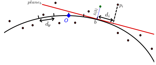
Figure 3: Computation of the height of the bin h(b) over the quadric surface using a local tangent plane at b , one of the bin of the patch. The center of the patch is marked with the blue diamond and named O .
