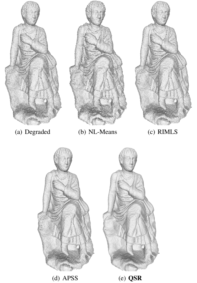
Figure 8: Groundtruth Comparison: super-resolution of an artificially degraded shape. The degradation involves a subsampling to 10% of the points and an additional Gaussian noise of variance 0.005% of the diagonal. Processing radius: r = 0.2 (Shape diagonal: 23.83), nbins_{lr} = 25 , nbins_{sr} = 100 , r_{sim} = 0.05 . Normals are computed using PCA with 10 neighbors for visualization purpose.
