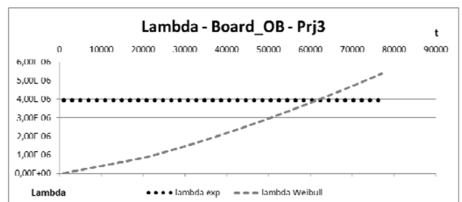
Figure 6. Comparison of Failure Rates for Prj3
