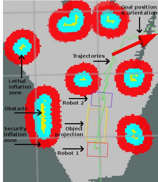
Fig. 7. Map of the starting and ending positions with obstacles, lethal and security inflation zones around them, the Nao and object footprints and goal position/orientation.
