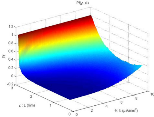
Fig. 11. Probability of failure based on degradation level (\rho_i, \theta_i) .
