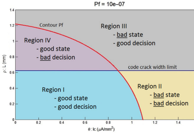
Fig. 12. Bivariate decision plan and a comparison with a mono-variate plan.
