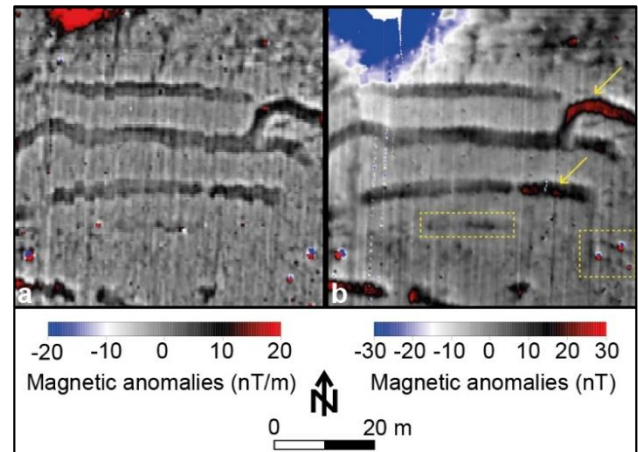
Fig. 6. Comparison between the magnetic maps obtain with the FEREX gradiometer composed by four fluxgate sensors (a) and with the G-858 magnetometer composed by two caesium vapour sensors (spaced horizontally) (b). The positioning of magnetic measurements of the G-858 magnetometer is carried out by the motorised total station.
