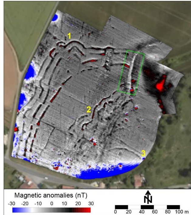
Fig. 4. Map of magnetic anomalies obtained using G-858 magnetometer. The prospected area, about 5ha, was mapped in four days. (1) external enclosure composed by four ditches ; (2) middle enclosure composed by two ditches ; (3) internal enclosure composed by one ditch. Green square shows the zig-zag effect induce by the relief (corresponding to a palaeo-cliff).
