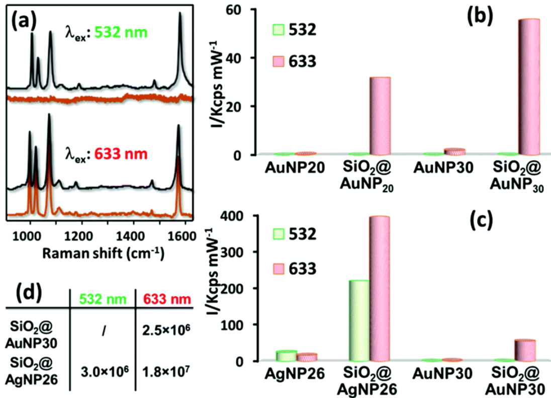
Fig. 10 (a) Representative SERS spectra of thiophenol (TP) on the raspberries-like cluster suspensions at various excitation wavelengths (532 and 633 nm) (gray: SiO 2 @AgNP26; orange red: SiO 2 @AuNP30). The spectra were rescaled for the sake of comparison. (b) and (c) Comparison of the SERS intensities of the TP band at 999 cm -1 for SERS spectra acquired at different excitation wavelengths on negatively charged colloids (AgNP26, AuNP20 and AuNP30) and their corresponding raspberry-like nanoclusters, based on polyelectrolyte-modified silica cores. SERS measurements were performed on the colloidal solutions and the corresponding SERS intensities were normalized to 1 s exposure time and 1 mW of laser power. The clusters concentration in the samples remained constant at ca. 6 \times 10^{13} L -1 . (d) Estimated SERS enhancement factors for SiO 2 @AuNP30 and SiO 2 @AgNP26 at different excitation wavelengths.
