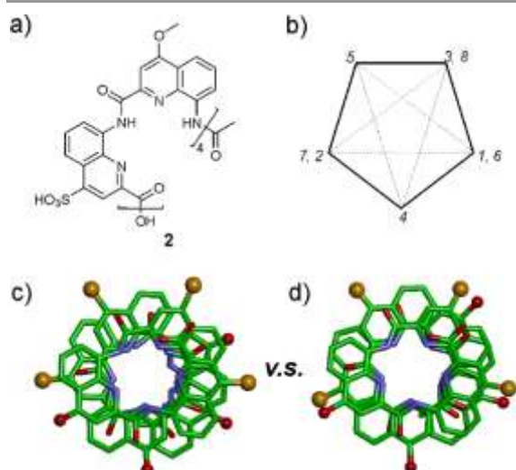
Figure 5. (a) Formula of octamer 2 . (b) Five-pointed star showing the usual positions of side chains in quinoline-based helices counting monomers from 1 to 8. Top views of the crystal structure of 2 (c), and of 6 (d) in which carboxylic acid side chains have been replaced by the side chains of 2 . All side chains are shown as golden (sulfonic acid) or red balls (methoxy).
