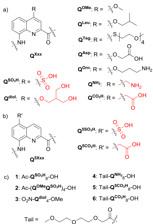
Figure 1. Structures of (a) Q^{xxx} and (b) Q^{5xxx} amino acid monomers, and summary of (c) aromatic amide foldamer sequences 1 - 6 . New side chains developed in this study are shown in red. The terminal 8-nitro group of oligomer 3 replaces the terminal NH function.
