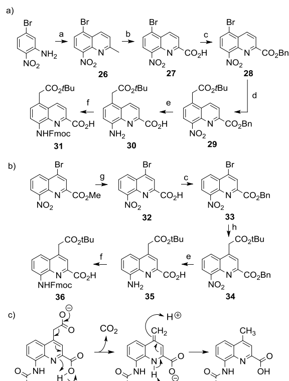
Scheme 4. Synthesis of a) Fmoc-Q CO2(tBu) -OH ( 31 ) and b) Fmoc-Q CO2(tBu) -OH ( 36 ). Reagents and conditions: (a) Ethylvinylether, H 2 SO 4 , AcOH, 70 °C to 120 °C, 30min; (b) SeO 2 , pyridine, 80 °C, 2d; (c) Benzyl bromide, K 2 CO 3 , DMF, r.t., 12h; (d) 2- tert -butoxy-2-oxoethyl zinc (II) bromide, bis(dibenzylidene acetone)-palladium [0], 1,2,3,4,5-pentaphenyl-1'-(di- tert -butylphosphino)ferrocene, THF, 70 °C, 12h; (e) H 2 , Pd/C, THF, r.t., 1d; (f) Fmoc-Cl, dioxane/H 2 O, 0 °C to r.t., overnight; (g) LiOH, THF/H 2 O, r.t., 1h; (h) 2- tert -butoxy-2-oxoethyl zinc (II) bromide, bis(dibenzylidene acetone)-palladium [0], 1,2,3,4,5-pentaphenyl-1'-(di- tert -butylphosphino)ferrocene, anhydrous THF, r.t., 4h. c) Possible decarboxylation mechanism.
