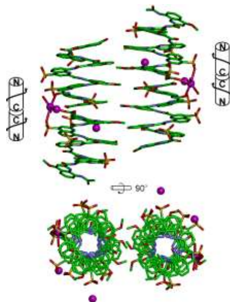
Figure 4. Crystal structure of 2 . Carbon, nitrogen, and oxygen atoms are shown in green, blue, and red, respectively. Calcium is shown as purple balls. Hydrogen atoms have been omitted for clarity. C- and N-termini and helix handedness are indicated in cartoons.
