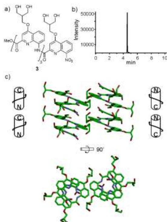
Figure 2. Formula (a), RP-HPLC chromatogram (b) and crystal structure (c) of 3 . Carbon, nitrogen and oxygen atoms are shown in green, blue and red, respectively. Hydrogen atoms have been omitted for clarity. C- and N-termini and helix handedness are indicated in cartoons.
