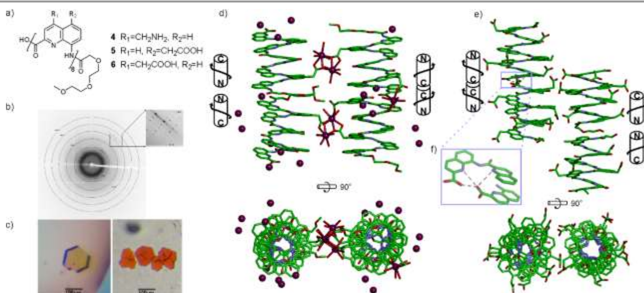
Figure 3. (a) Formulae of octamers 4-6 . Diffraction pattern (b) and crystals (c) of 4 . Crystal structures of 5 (d) and 6 (e-f). In (d), some side chains have been omitted for clarity. Hydrogen bonds (dashed grey lines) connect two stacked helices of 6 at their C-termini (f). Carbon, nitrogen, and oxygen atoms are shown in green, blue, and red, respectively. Calcium is shown as purple balls. Hydrogen atoms have been omitted for clarity. C- and N-termini and helix handedness are indicated in cartoons.
