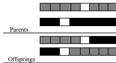
Fig.5. Single point crossover
