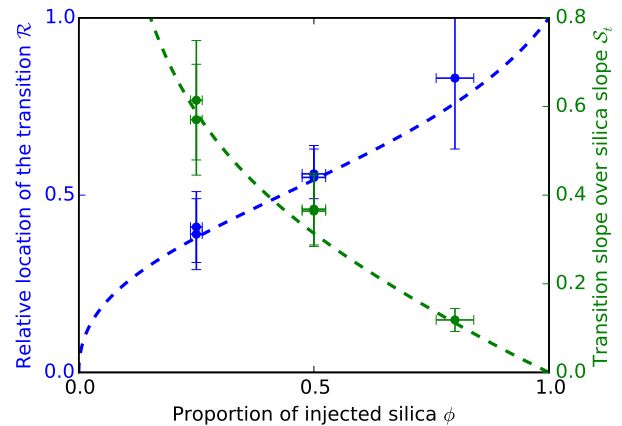
Figure 14. Relative position of the transition \mathcal{R} (blue) and dimensionless transition slope S_t (green), as a function of the composition of the sediment input. Dots: experimental measurements. Dashed lines: Eqs. (9) and (10) with S = 3.4 .
