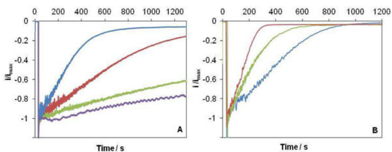
Figure 5. Kinetics of O_2 reduction inhibition by NaCl. Chronoamperometric measurement at E = +0.3 V vs. Ag/AgCl (A) as a function of pH at T = 37^\circ\text{C} and 50 mM NaCl: pH 4 (blue curve), pH 5 (red curve), pH 6 (green curve) and pH 7 (purple curve); (B) as a function of temperature at pH 4 and 50 mM NaCl: T = 25^\circ\text{C} (blue curve), T = 37^\circ\text{C} (green curve), T = 50^\circ\text{C} (red curve). O_2 -saturated 200-100 mM phosphate-citrate buffer. Electrodes modified as in Fig 1.
