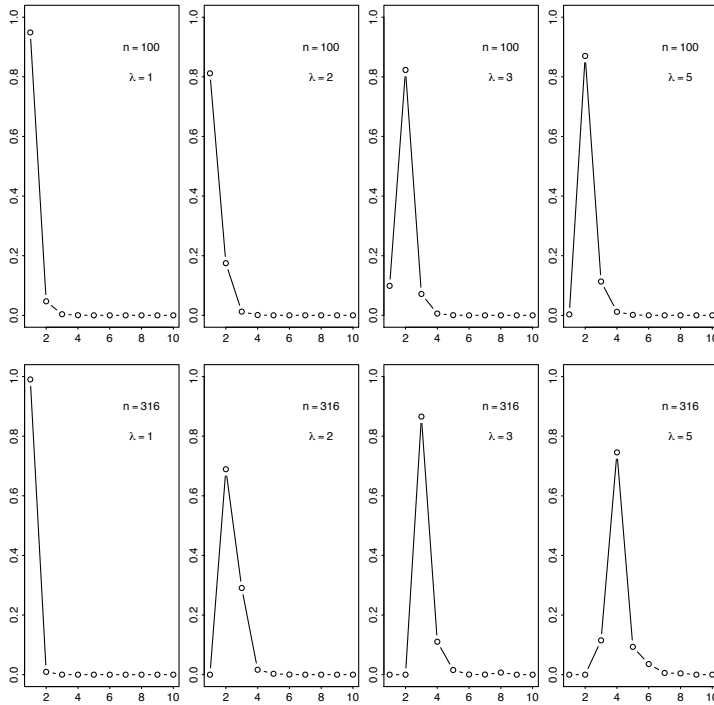
Fig. 2 Approximate posterior distribution \hat{p}(Q|\mathbf{X}) of the number Q \in \{1, \dots, 10\} of classes in the SBM model, for \rho = 10^{-1.5} and various values of n as well as \lambda .
