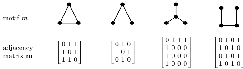
Fig. 8 Adjacency matrix \mathbf{m} for four typical motifs.
