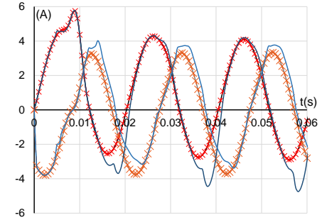
Fig. 6. Evolutions of the current associated with two primary windings for resistor load ( R=200\Omega ).
