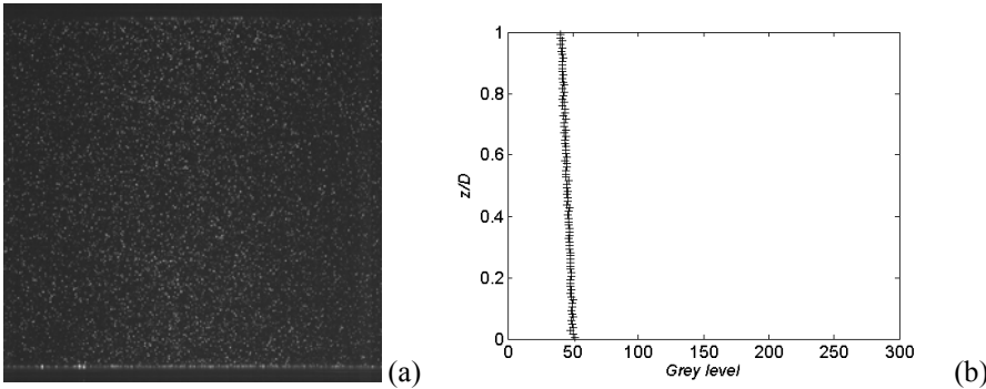
Figure 3: Single phase flow (a) PIV raw image (b) vertical grey level profile ( U_m=1.2\text{m/s} )
