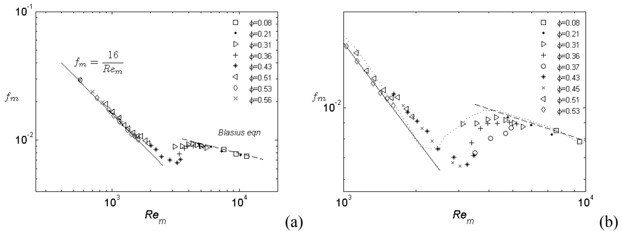
Figure 15: (a) Wall friction factor as a function of the Reynolds number, (b) Zoom of the transition region including Nikuradse experimental data (...)
