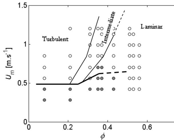
Figure 6: Flow pattern map (○): homogeneous flow, (●): partially stratified flow. Thin lines separate the flow regime domains. Thick line is the approximate limit between the homogeneous (above) and the partially stratified configuration (below)
