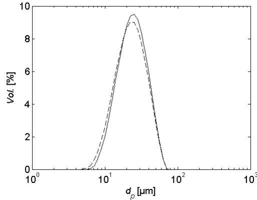
Figure 2: Drop size distribution for \phi=0.08 (—) and \phi=0.12 (---)
