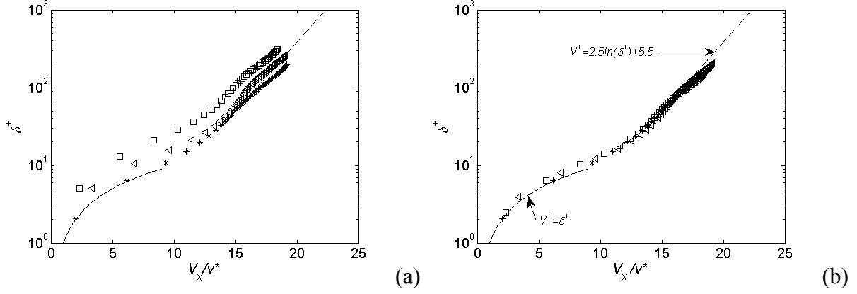
Figure 8: Wall law velocity. Single phase flow (*) : ( U_0=0.42\text{m/s} , Re_\sigma=7200 , V_{x\text{max}}=0.54\text{m/s} ); Two-phase flow ( \triangleleft ) : ( \phi=0.08 , U_m=0.56\text{m/s} , V_{x\text{max}}=0.72\text{m/s} ), ( \square ): ( \phi=0.21 , U_m=0.85\text{m/s} , V_{x\text{max}}=1.1\text{m/s} ). (a) \delta normalized by continuous phase properties, \mu_c and \rho_c (b) \delta normalized by mixture properties, \mu_m and \rho_m
