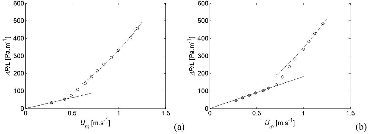
Figure 13: Pressure drop as a function of U_m (a) \phi=0.31 (b) \phi=0.36 , (—) dP/dx \propto U_m (---) dP/dx \propto U_m^{1.75}
