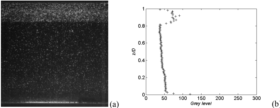
Figure 5: Partially stratified flow (a) PIV raw image (b) vertical grey level profile ( \phi=0.21 , U_m=0.28\text{ m/s} )
