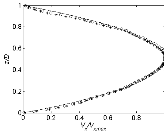
Figure 10: Normalized velocity profile at \phi = 0.53 , (*) U_m = 0.56\text{m/s} ( V_{x\max} = 1.1\text{m/s} ), (o) U_m = 0.7\text{m/s} ( V_{x\max} = 1.3\text{m/s} ), (—) parabolic profile
