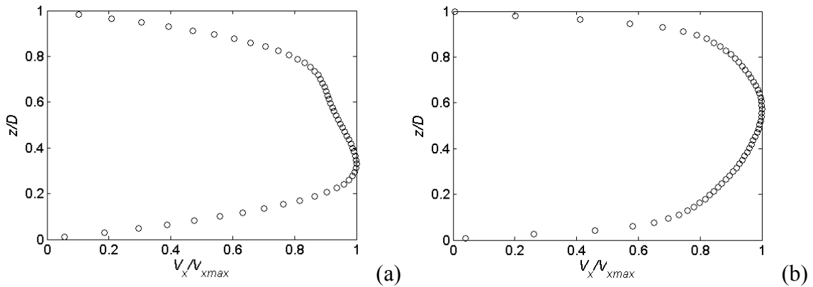
Figure 12: Axial velocity profile (a) \phi = 0.43 , U_m = 1.2 \text{m/s} , V_{xmax} = 1.8 \text{m/s} (b) \phi = 0.37 , U_m = 1.2 \text{m/s} , V_{xmax} = 1.6 \text{m/s}
