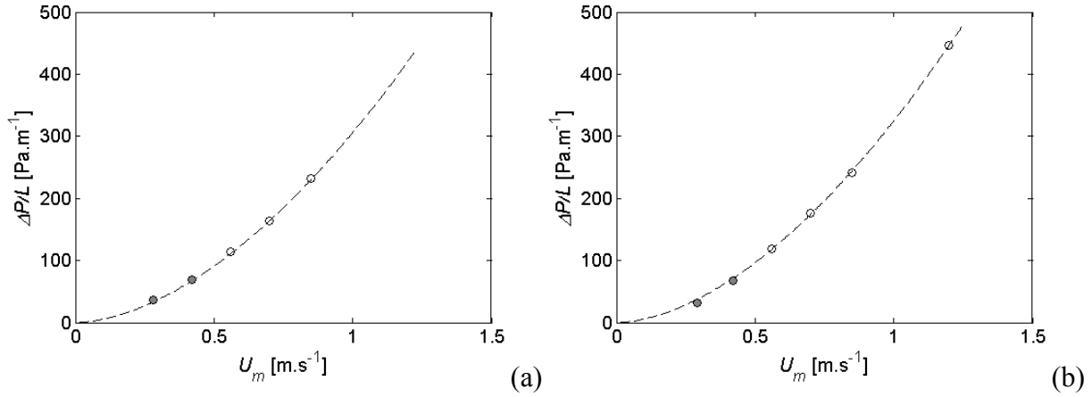
Figure 9: Evolution of the pressure drop as a function of the mixture velocity for (a) \phi=0.08 , (b) \phi=0.21 . Solid symbols correspond to partially homogeneous profiles. Dashed line corresponds to Eq. 9.
