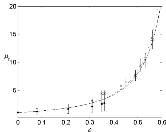
Figure 14: Relative viscosity as a function of oil volume fraction ( \phi_m = 0.74 ), (...) Eilers, (- - -) Krieger and Dougherty. (●) Blasius friction factor (×) Hagen-Poiseuille friction factor
