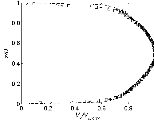
Figure 7: Normalized longitudinal velocity profile. Single phase flow (*) : ( U_0=0.42\text{m/s} , Re_\theta=7200 , V_{xmax}=0.54\text{m/s} ); Two-phase flow ( \triangleleft ) : ( \phi=0.08 , U_m=0.56\text{m/s} , V_{xmax}=0.72\text{m/s} ), ( \square ): ( \phi=0.21 , U_m=0.85\text{m/s} , V_{xmax}=1.1\text{m/s} ); (---): V_x/V_{xmax} = (1 - 2|z/D - 1/2|)^{2/13}
