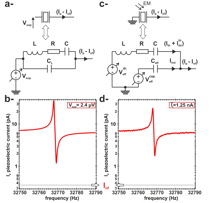
FIG. 7: (Color online) a-Butterworth-Van Dyke circuit used to describe the QTF when electrically actuated by an external supply ( V_{sup} ). b-5Spice ® simulation of the TF of the Butterworth-Van Dyke circuit shown in a-. The R , L , C parameters are those formerly derived for our QTF and the I/V converter TF was included in the simulation. To achieve a background current of \simeq 7 pA, consistently with the experimental spectrum shown in d-, we need to input V_{sup} = 2.4 \mu V . The resonance/anti-resonance behavior is well-known with this kind of circuit. c-Equivalent circuit of the QTF upon EM excitation. The Butterworth-Van Dyke circuit is reconsidered. The two branches are separated and excited by independent effective voltage sources. d-Experimental I_p(f, \tilde{I}_t) spectrum reported from fig.5b for \tilde{I}_t = 1.25 nA. The resonance/anti-resonance behavior is qualitatively similar as the one shown in b-.
