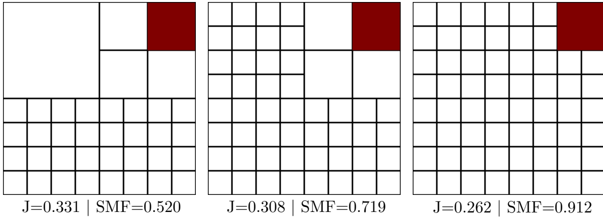
Fig 11 Illustration of several decomposition examples with the corresponding average binary shape in red, and J (10) and \text{SMF} (15) values.
