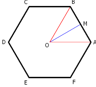
FIGURE A.1. The hexagon \mathcal{H}
