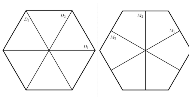
FIGURE 7.3. The lines of symmetry of the hexagon
