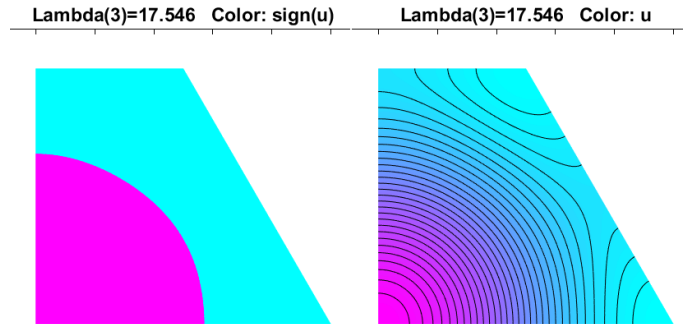
FIGURE 7.8. Nodal pattern for \mu_3(\mathcal{R}, \mathbf{nnn})
