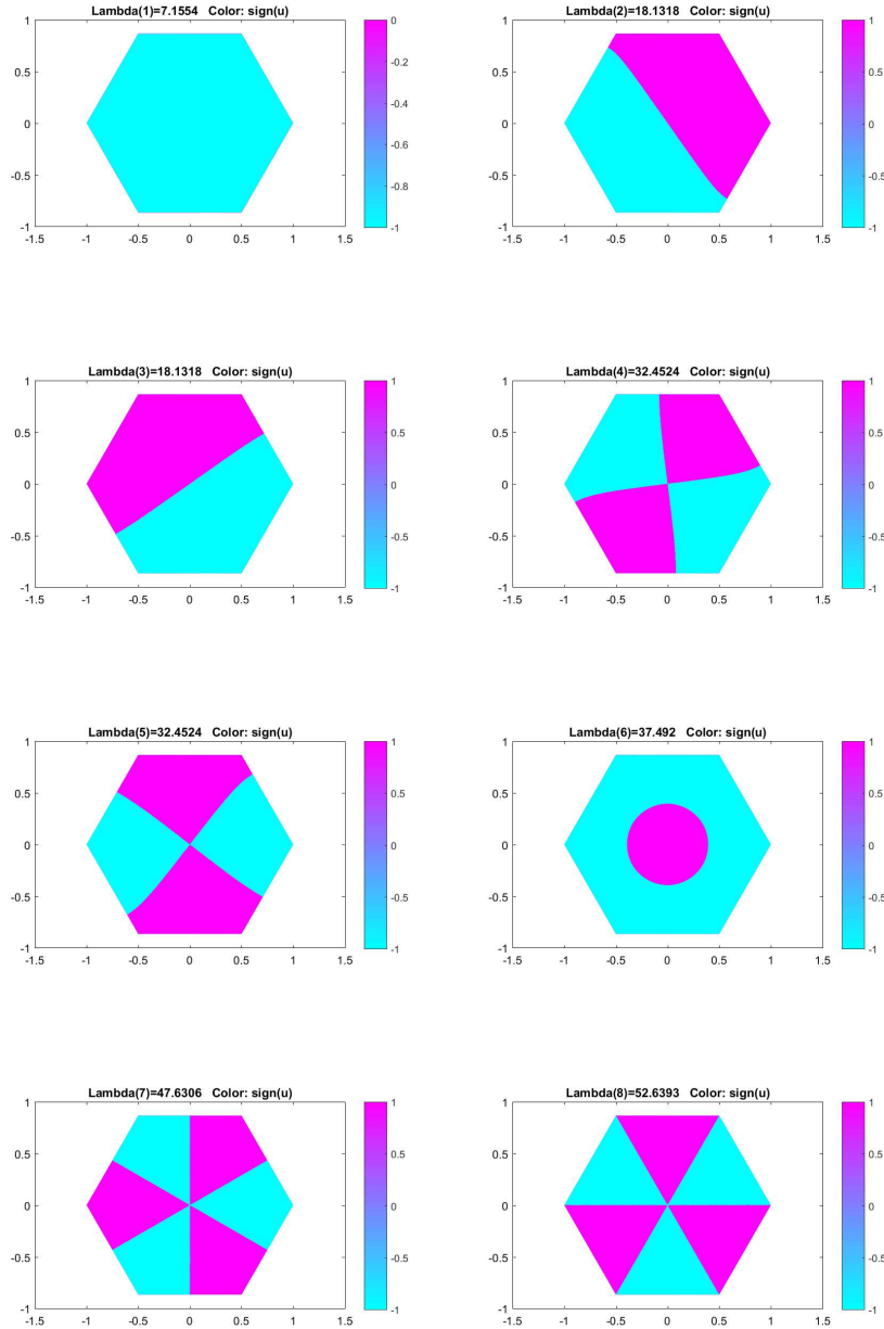
FIGURE 7.5. Eigenpairs for the hexagon with Dirichlet condition using MATLAB
