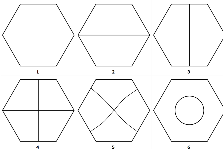
FIGURE 7.4. Nodal structure for the six first eigenfunctions of the Dirichlet Laplacian in the hexagon
