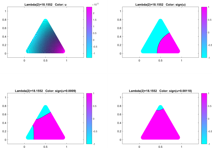
FIGURE 6.3. Level sets of one of the second Neumann eigenfunctions of the equilateral triangle with rounded corners
