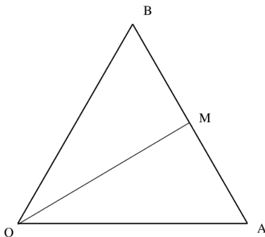
FIGURE 6.1. Equilateral triangle \mathcal{T}_e = [OAB]
