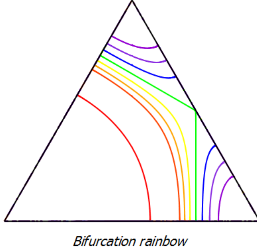
FIGURE 6.2. Level sets \{\varphi_2^N + a = 0\} for a \in \{0; 0.7; 0.8; 0.9; 1; 1.1; 1.2; 1.3\}
