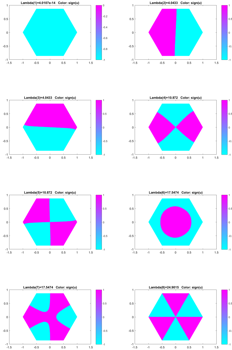
FIGURE 7.6. Eigenpairs for the hexagon with Neumann condition using MATLAB
