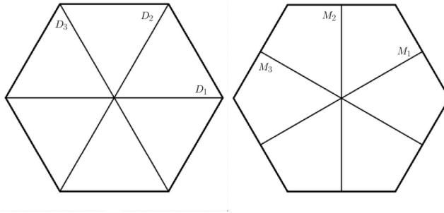
FIGURE 7.2. The lines of symmetry of the hexagon
