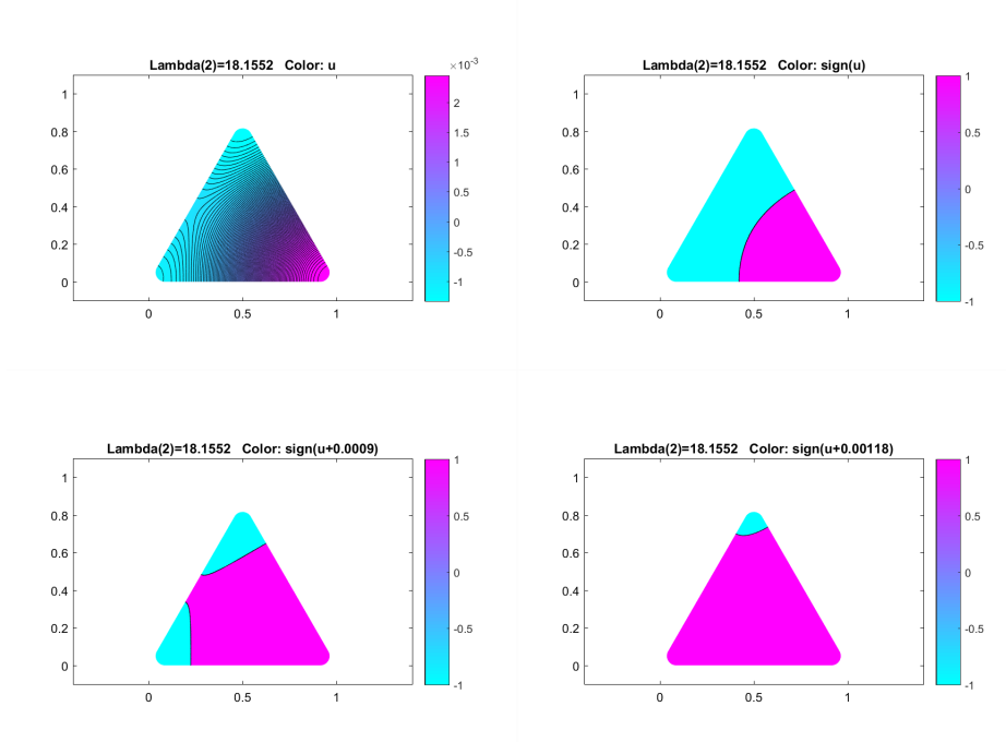
FIGURE 6.3. Level sets of one of the second Neumann eigenfunctions of the equilateral triangle with rounded corners
