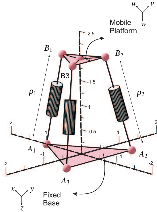
Fig. 1. 3-RPS parallel robot
