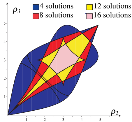
Fig. 7. Slice of the joint space for \rho_1 = 3 and the number of solution for DKP for k = 1
