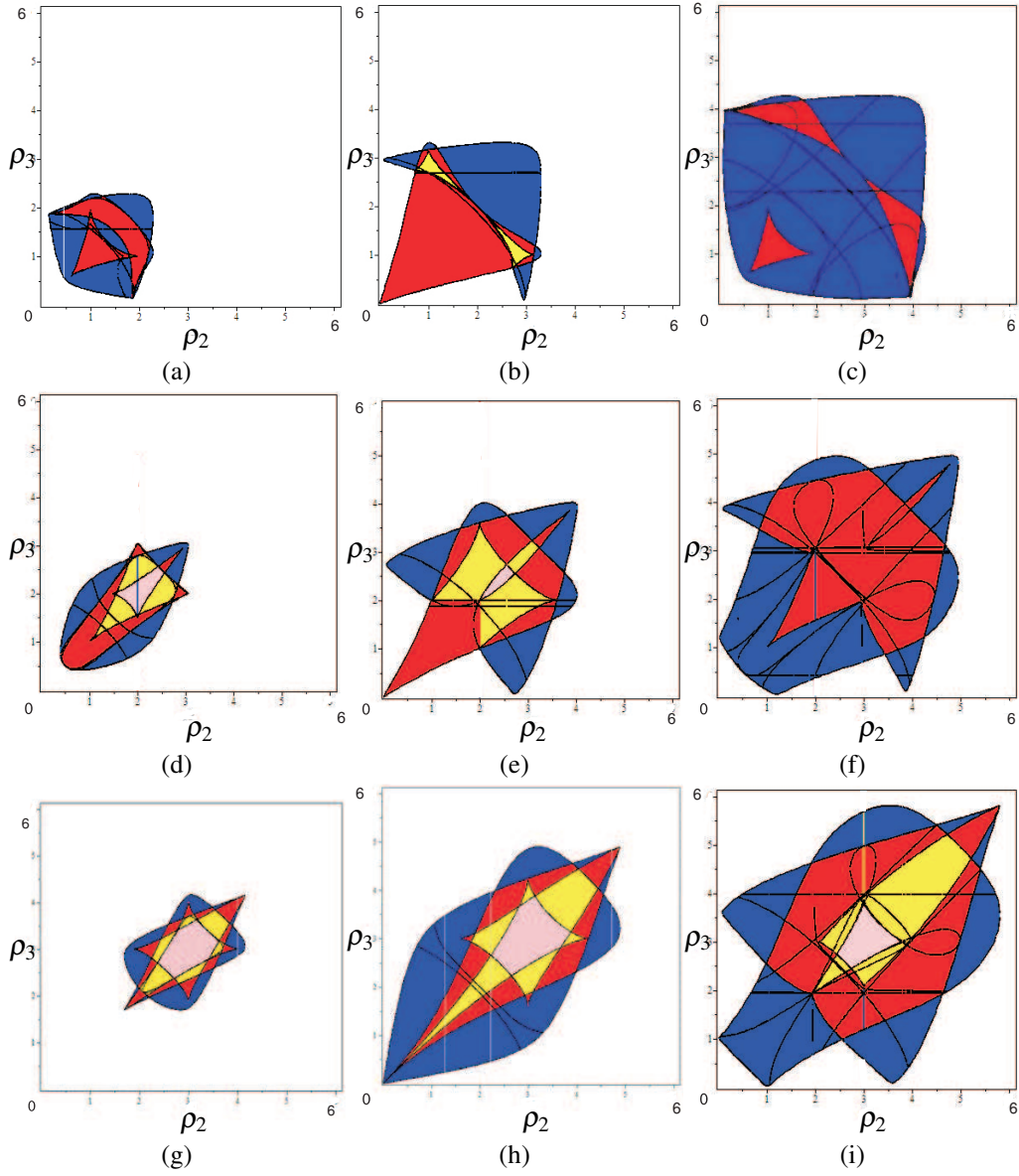
Fig. 6. Slice of the joint space for \rho_1 = 1, k = 0.5 (a), \rho_1 = 1, k = 1 (b), \rho_1 = 1, k = 1.5 (c), \rho_1 = 2, k = 0.5 (d), \rho_1 = 2, k = 1 (e), \rho_1 = 2, k = 1.5 (f), \rho_1 = 3, k = 0.5 (g), \rho_1 = 3, k = 1 (h) \rho_1 = 3, k = 1.5 (i), where the DKP admits four, eight, twelve and sixteen real solutions in the blue, red, yellow and pink region, respectively.
