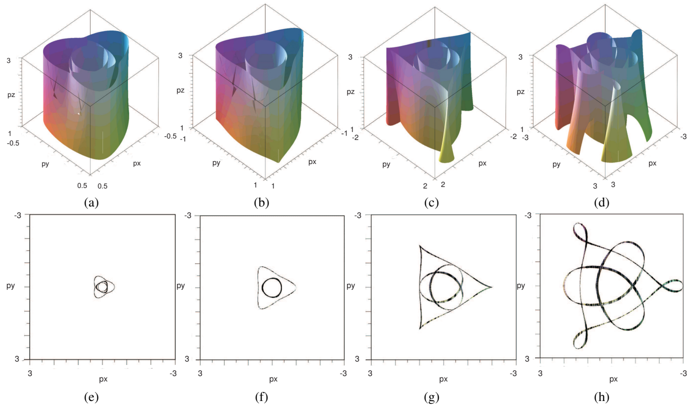
Fig. 3. Projection of parallel singularities in projection space [p_x p_y p_z] for OM^1 . Variation in the parallel singularities surface for different design parameter k = 0.5 (a), k = 1 (b), k = 2 (c) and k = 3 (d), top view of the parallel singularities surface, k = 0.5 (e), k = 1 (f), k = 2 (g) and k = 3 (h).
