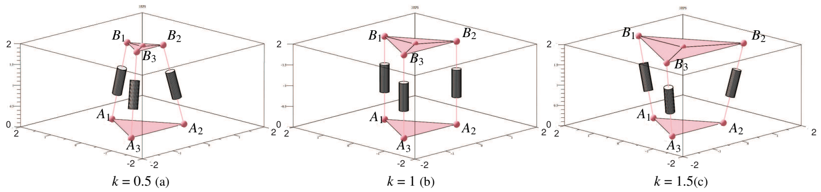
Fig. 2. Virtual model of 3-RPS parallel manipulator with different design parameter k , k = 0.5 (a), k = 1 (b), k = 1.5 (c)
