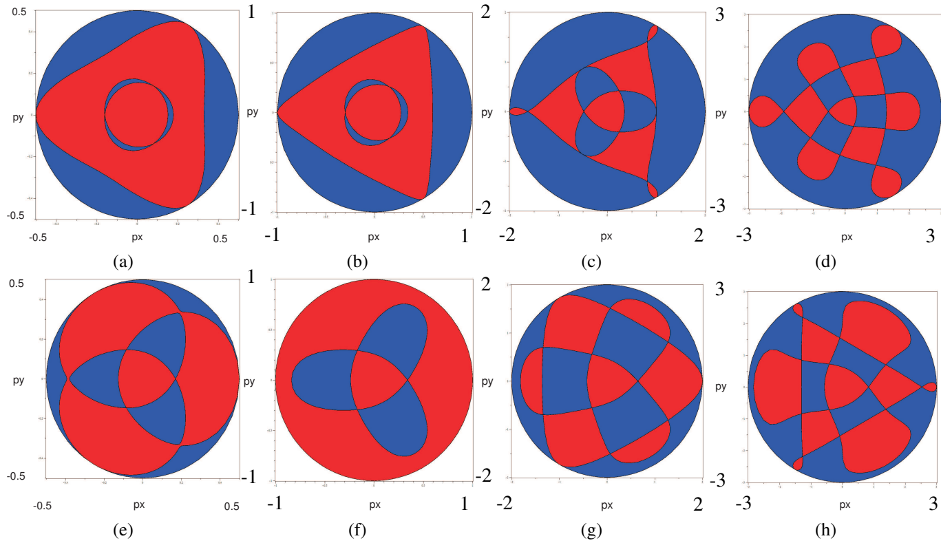
Fig. 5. Slice of workspace for OM^1 with different design parameter and p_z = 2 , k = 0.5 (a), k = 1 (b), k = 2 (c) and k = 3 (d) for OM^2 k = 0.5 (e), k = 1 (f), k = 2 (g) and k = 3 (h). Blue and red regions corresponds to the four number of solutions for the IKP for \det(\mathbf{A}) > 0 and \det(\mathbf{A}) < 0 , respectively.
