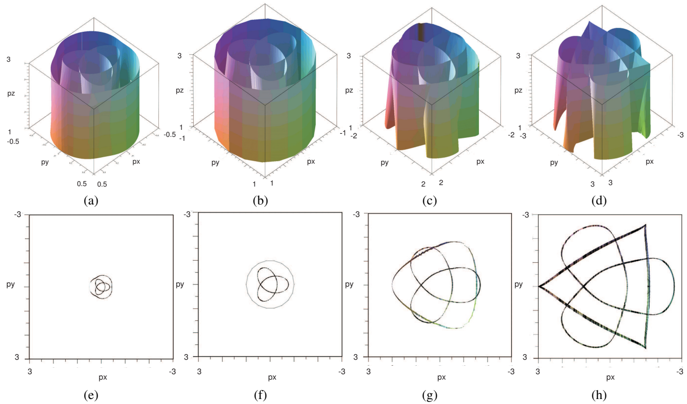
Fig. 4. Projection of parallel singularities in projection space [p_x, p_y, p_z] for OM^2 . Variation in the parallel singularities surface for different design parameter k = 0.5 (a), k = 1 (b), k = 2 (c) and k = 3 (d), top view of the parallel singularities surface, k = 0.5 (e), k = 1 (f), k = 2 (g) and k = 3 (h).
