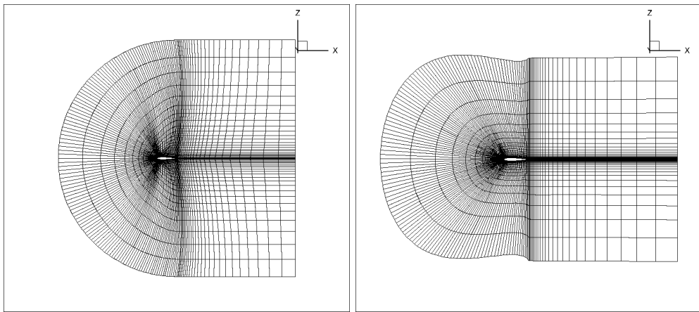
Figure 5: Parabolic mesh around the profile. Figure 6: Hyperbolic mesh around the profile.
