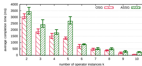
Fig. 2: Prototype average per tuple completion time \bar{L}^{alg} as a function of the number of operators k .
