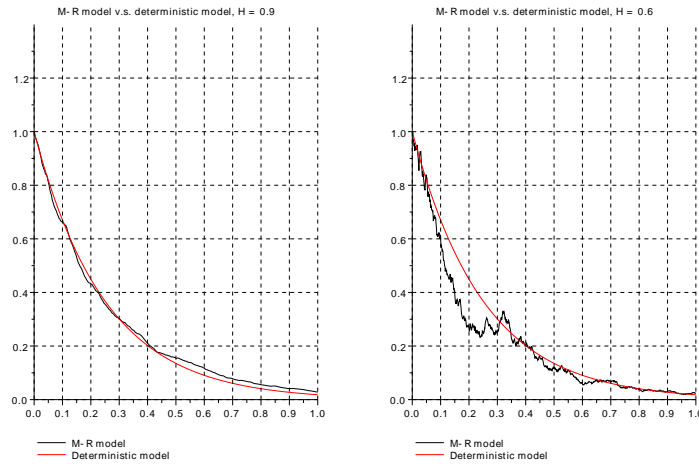
FIGURE 1. GM-R model v.s. deterministic model currently used
