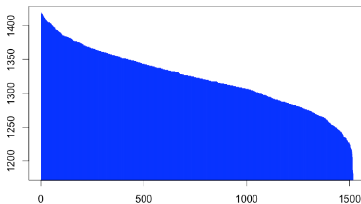
Fig. 6. Robust RSOM : fickle words with the number of their fickle pairs
