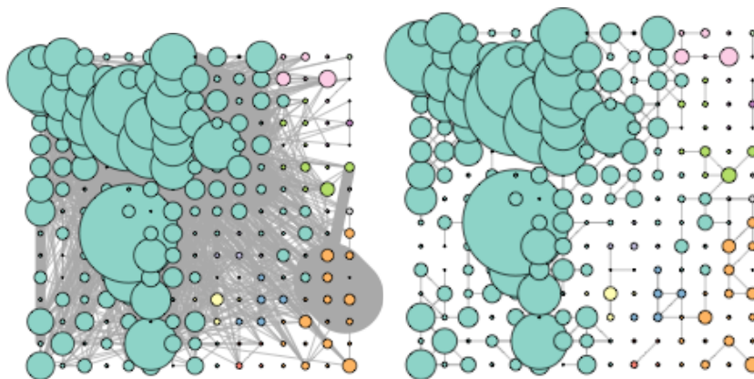
Fig. 5. Robust Korresp : projected graph. Left : only the edges with weights larger than the mean weight value are drawn. Right : only the edges of the four nearest neighbors - left, right, below, above - are drawn. The radius of the clusters is proportional to their size; the width of the edges is proportional to their weight
