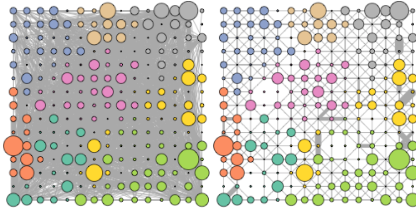
Fig. 9. Robust RSOM : projected graph. Left : only the edges with weights larger than the 3rd quartile are drawn. Right : only the edges of the four nearest neighbors - left, right, below, above - are drawn. The radius of the clusters is proportional to their size; the width of the edges is proportional to their weight
