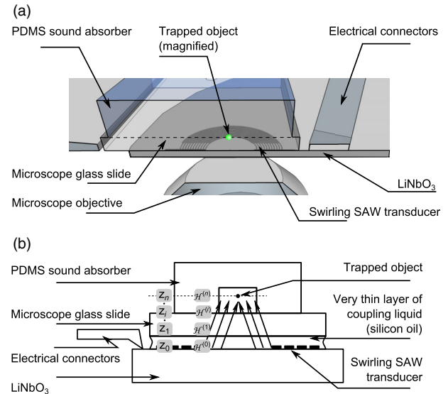
FIG. 2. PSR-based acoustical tweezers integrated in a microscope for particle manipulation. The transducer is a pair of spiraling interdigitated gold electrodes deposited on a piezoelectric substrate. A microscope slide is placed on the transducer, and acoustic transmission is ensured by the mean of a thin layer of silicon oil. An aqueous suspension of micrometric polystyrene beads is dispersed between the microscope slide and an upper layer of PDMS that plays the role of acoustic absorber. The center of the vortex is visualized by a reticule. The device is represented (a) at the top, while (b) the bottom provides a more schematic cross section.
