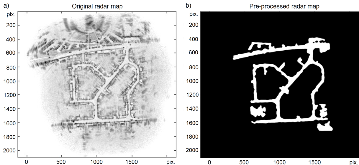
Figure 6: Retrieval of the roads in the radar map: a) Original radar map (resol.: 20cm) ; b) Result of the processing (gray-level thresholding, retrieval of the major boundaries and median filtering).
