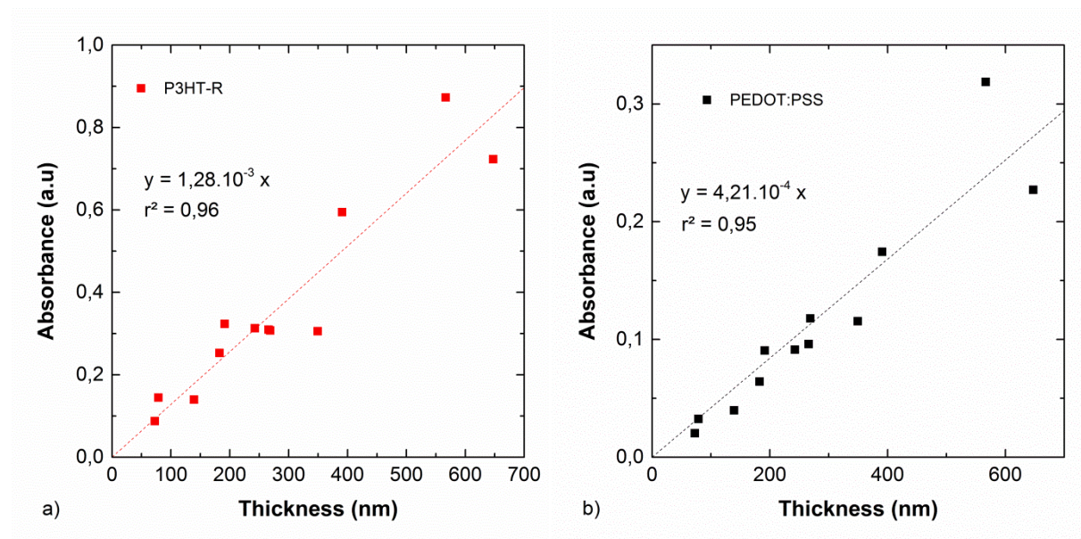
Figure A: Absorbance values of P3HT-R and PEDOT:PSS from (\text{P3HT-R/PEDOT:PSS})_n multilayer films as a function of their thickness. a) 450 nm for P3HT-R, b) 930 nm for PEDOT:PSS.
