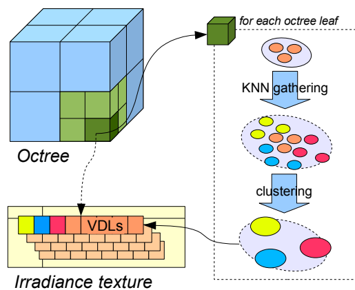
Figure 3: Octree clustering
