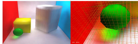
Figure 11: Caustics rendering
