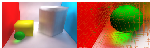
Figure 11: Caustics rendering
