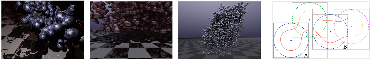
(a) Raytracing of metaballs, with shadows and 3 levels of mirror reflections: (left) 1000 metaballs at 13 fps at a 640 \times 480 resolution without multi-sampling; (center) 200K metaballs at 0.3 fps at 1600 \times 1200 with 4 rays per pixel; (right) 3000 metaballs at 1.1 fps at 1600 \times 1200 with 4 rays per pixel.
