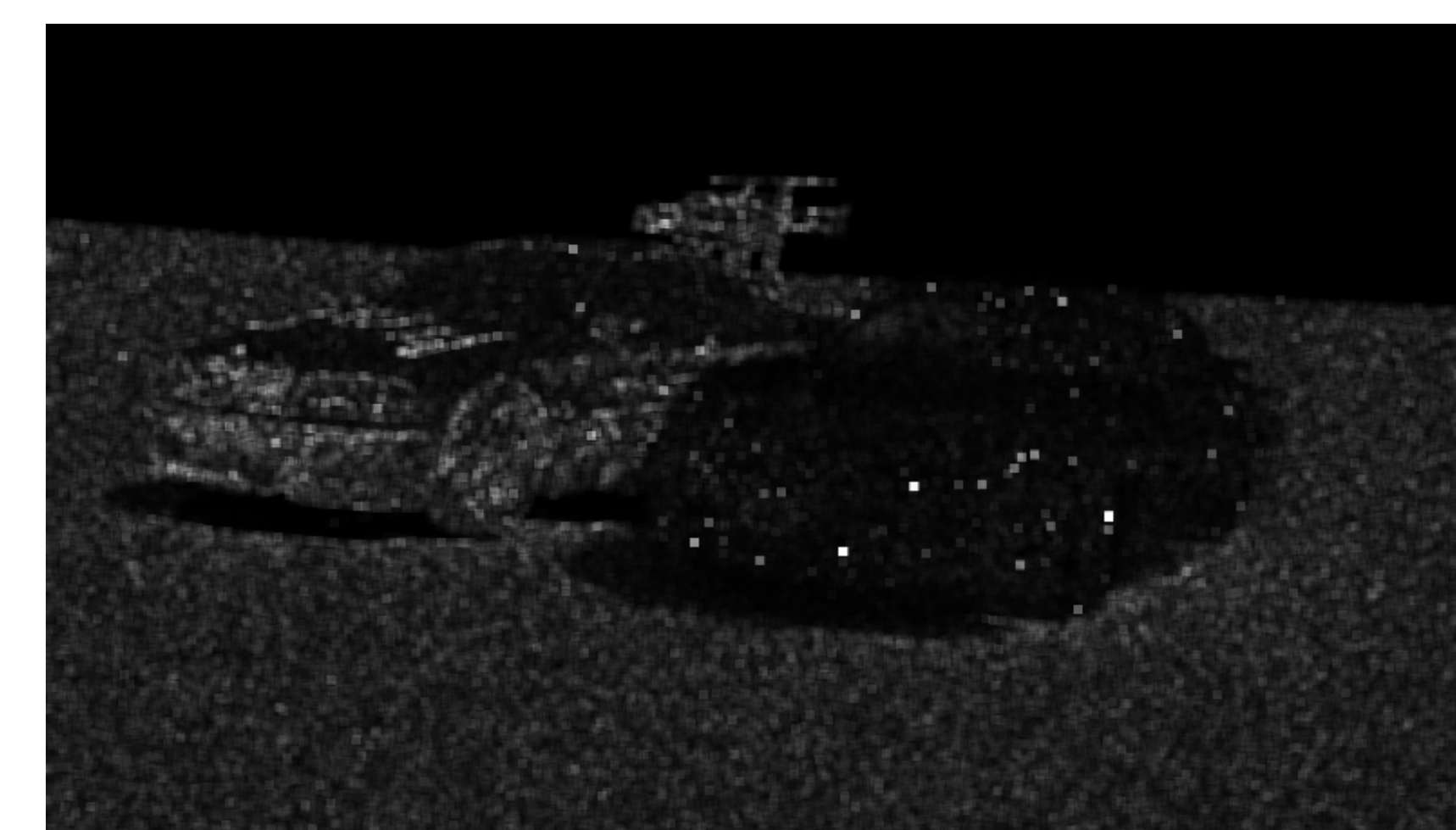
Noise measure for Tsallis entropy
