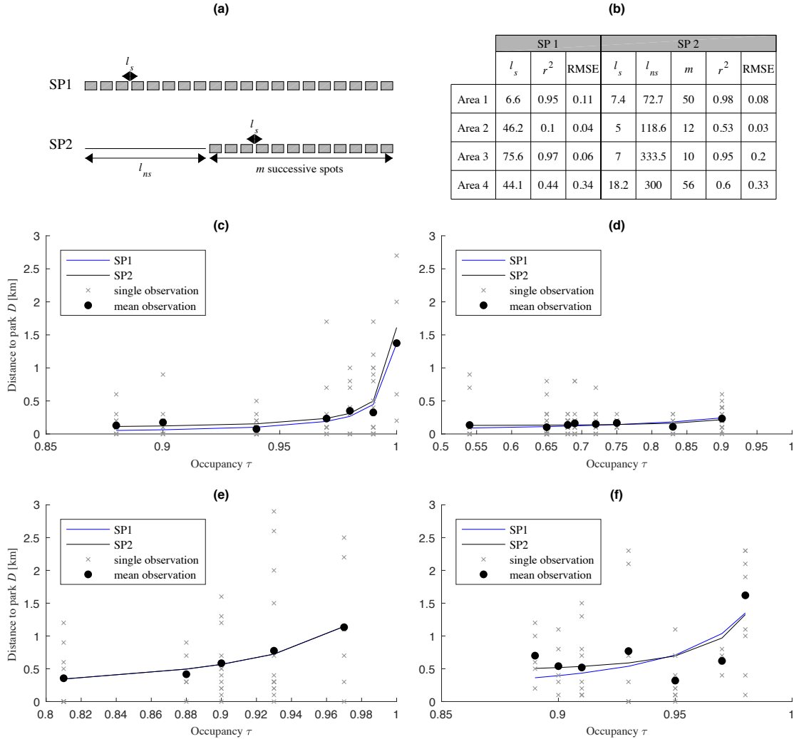
Figure 1: On-street parking search process (a) SP1 vs. SP2 parking processes (b) synthesis of calibration results (c) to (f) calibration results for areas 1 to 4.
