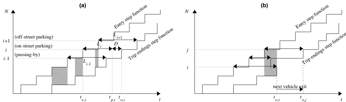
Figure 3: Event-based resolution of the trip-based MFD model (a) general principle (b) FIFO exit times with respect to the original exit time order
