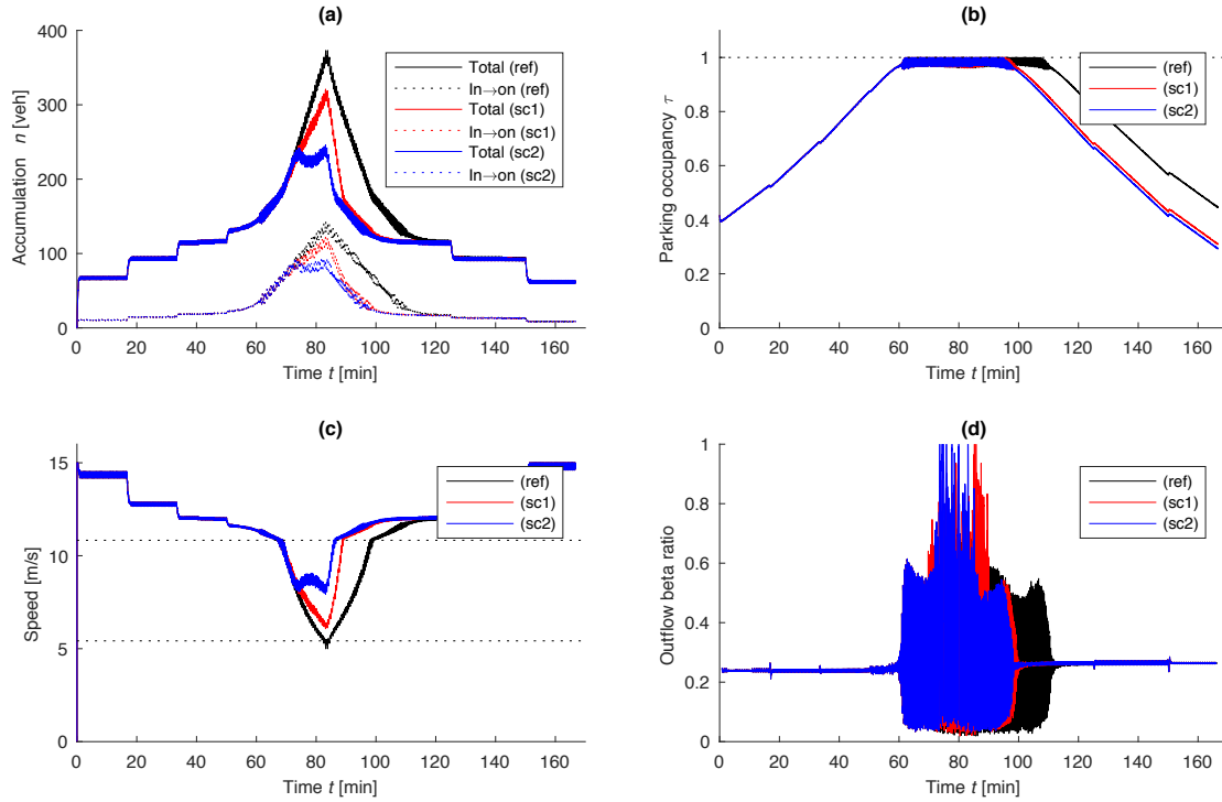
Figure 7: Simulation results for two reactive feedback strategies on the parking demand (a) time-evolution of the total and In-to-on accumulations (b) time-evolution of the on-street parking occupancy (c) time-evolution of the mean network speed (d) time-evolution of the outflow beta ratio.
