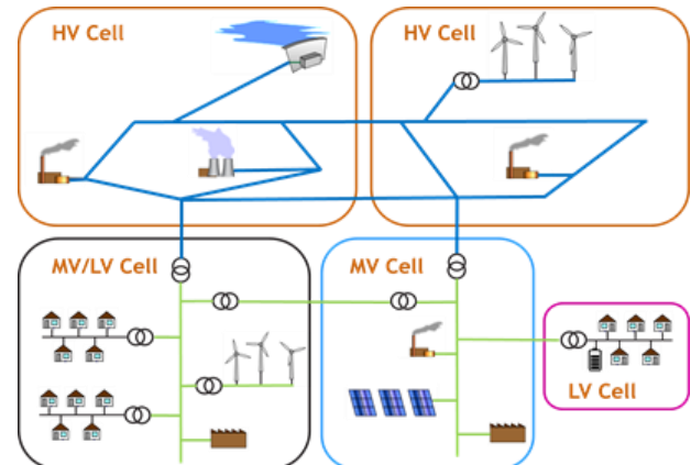
Figure 2: Schematic example of the proposed “Web-of-Cells” architecture
