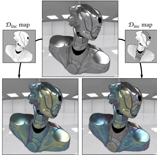
Fig. 13. The ROBOT model is made of a metallic base ( \alpha = 0.07 , \eta_3 = 1.87 , \kappa_3 = 1.182 ) to which we add a thin-film of index \eta_2 = 1.42 and varying thickness ( \mathcal{D}_{inc} \in [0..1125]\text{nm} ). On the left, we use an ambient occlusion texture to guide thickness variations. On the right we add regular patterns to guide a futuristic look. The image on top is rendered without iridescence.
