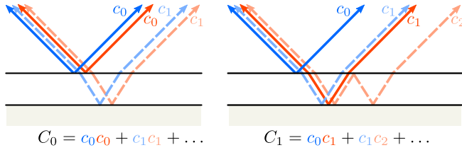
Fig. 6. We illustrate the C_m terms of Equation 5. Left: C_0 is obtained by summing interferences for all pairs of light paths of the same order. Right: C_1 is obtained by summing interferences for all pairs of light paths with an offset of m = 1 in orders.
