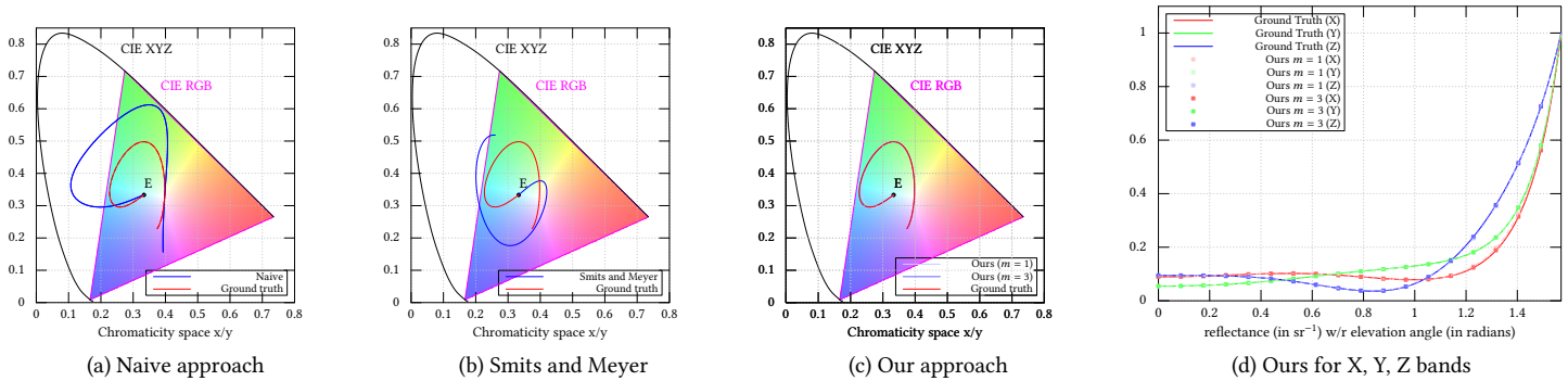
Fig. 7. We compare different approximations to a ground truth reflectance for a dielectric film ( \eta_2 = 1.5 ) of thickness d = 525\text{nm} over a dielectric base ( \eta_3 = 1.09 ). In (a-c), reflectance curves parametrized by \theta_1 are plotted in CIE xy chromaticity space, with the ground truth in red and approximate solutions in blue. The naive approach in (a) uses the exact Airy reflectance, but only one wavelength sample per spectral band, which yields poor results. The approach of Smits and Meyer [Smits and Meyer 1992] in (b) makes several simplifications to the reflectance model (e.g., \kappa_3 = 0 ); even with a dense spectral sampling identical to the ground truth, it still shows significant disparities. Our approach is shown in (c) for different truncations of the offset m . Computationally, it is only slightly more complex than the naive approach; yet it produces results nearly indistinguishable from the ground truth, as is also shown for each of the X, Y, and Z spectral bands in (d).
