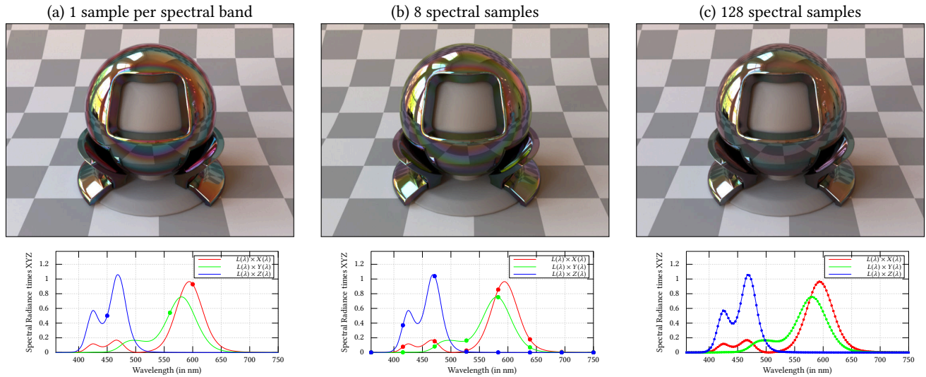
Fig. 2. The addition of a thin film layer requires a dense spectral sampling to render colors properly. We show this in the top row: (a) with only one sample per spectral band (as done in RGB rendering), colors appear unnaturally over-saturated; (b) 8 spectral samples produce different color patterns; (c) a reference using 128 samples per spectral band shows the correct colors. These color artefacts are due to spectral aliasing , as shown in the bottom row where spectral sampling is visualized for one surface point. The colored curves correspond to reflected radiance multiplied by either the CIE X, Y, or Z sensitivity curve, in red, green and blue respectively. They show oscillations that obviously cannot be captured with a single sample (a), or even 8 samples (b), hence yielding aliasing issues in these two cases. The use of 128 samples correctly captures these oscillations but is impractical when thin-film thickness, and hence reflectance, varies.
