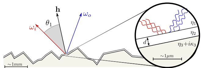
Fig. 3. Our reflectance model is composed of a micro-facet surface of complex index \eta_3 + i\kappa_3 with a thin dielectric film of index \eta_2 on top of each micro-facet. The small thickness d of the film requires to treat light interactions at the surface using wave optics.
