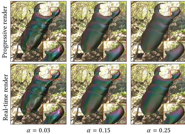
Fig. 16. The STAG BEETLE model is rendered with a dielectric base ( \eta_2 = 1.21 , \eta_3 = 2.0 , D_{inc} = 1740\text{nm} ) using progressive rendering in the top row, and a real-time approximation in the bottom row (see text). When the roughness \alpha of the base layer increases, the real-time approximation is less and less accurate; in particular, color fringes become over-saturated.
