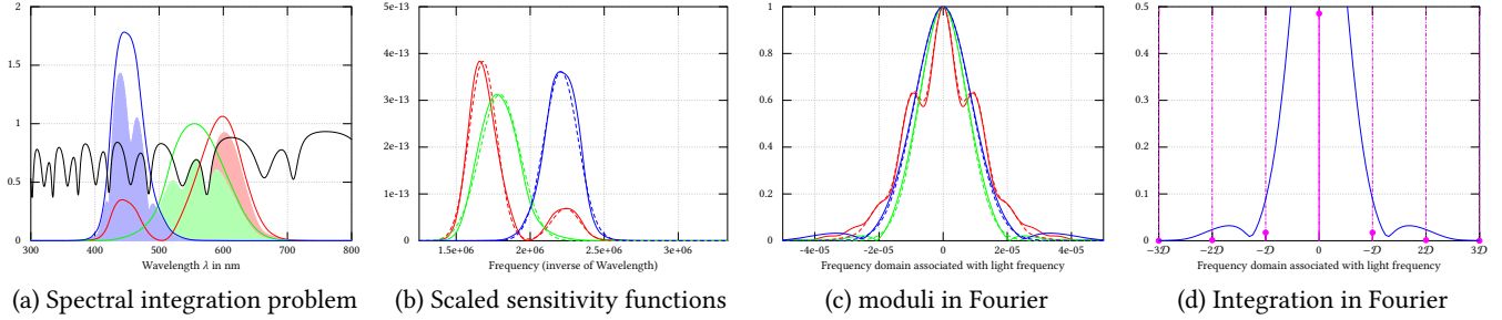
Fig. 5. The spectral integration problem is illustrated in (a) for the CIE XYZ color space: the reflectances \{R_X, R_Y, R_Z\} (light colored areas) are obtained by integrating the product of each sensitivity curve ( s_X in red, s_Y in green, s_Z in blue) with the spectral Airy reflectance R (in black). In our approach, the sensitivity functions are first re-expressed in terms of \nu = 1/\lambda in (b), yielding \{S_X, S_Y, S_Z\} . They are then transformed in Fourier space: the moduli \{|\hat{S}_X|, |\hat{S}_Y|, |\hat{S}_Z|\} are shown in (c). Since the Fourier transform \hat{R} of the Airy reflectance term is composed of diracs, the integral in Fourier becomes analytical as shown in (d) for the evaluation of R_Z . The dashed curves in (b) and (c) show Gaussian fits, which provide reasonable approximations in practice.
