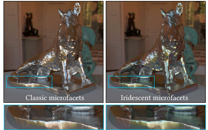
Fig. 17. We reproduce the subtle iridescent appearance of oxide layers on top metals with the BOAR model. Iridescence adds a touch of green and purple (right inset) to a base ‘white’ material (left inset). The base layer index is here given by \eta_3 = 1.5 and \kappa_3 = 3 , and the thin film is d = 600\text{nm} thick and has an index of \eta_2 = 1.33 .
