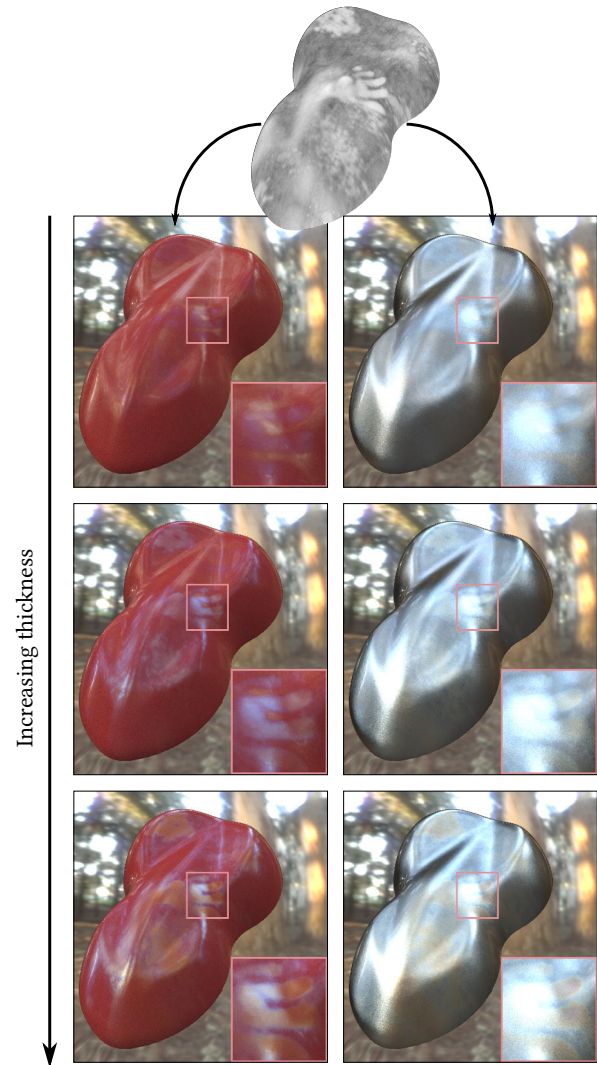
Fig. 12. The SPEEDSHAPE model is rendered with a dielectric base in the left column ( \alpha = 0.1 , \eta_2 = 1.25 , \eta_3 = 1.72 , \rho_d = \{0.191, 0.015, 0.015\} ) and a rough conductor base in the right column ( \alpha = 0.18 , \eta_2 = 1.25 , \eta_3 = 1.1 , \kappa_3 = 1.63 ). The thin-film of spatially-varying thickness is revealed by remapping \mathcal{D}_{\text{inc}} from 0 to 100nm (first row), to 200nm (second row), and to 400nm (third row), controlled by the texture shown on top.
