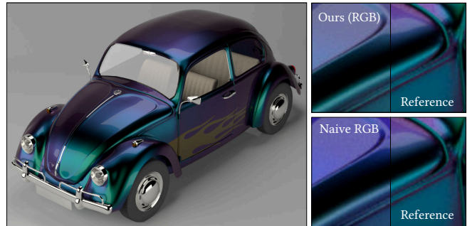
Fig. 18. With the BEETLE model we tried to reproduce the look of special effet car paints (see our supplemental video for an example). We show that even for a configuration where the variation of colors is moderate and dense sampling is probably not required, the naive RGB model still produces inaccurate colors. Here we used a conducting base layer ( \eta_3 = 1.2 , \kappa_3 = 0.5 ) with a thin-film of d = 505\text{nm} and index \eta_2 = 1.39 . We also added a clear coat of \eta_1 = 1.2 to further match the car paint appearance. The door-side sticker is created by varying thickness using a texture.
