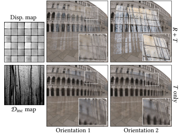
Fig. 14. Our model works with transparent objects, here a transparent slab obtained by applying a displacement map to a plane, with a rough dielectric base ( \alpha = 0.2 , \eta_3 = 1.45 ). We control variations of the thin-film ( \eta_2 = 2.0 ) using a texture that remaps \mathcal{D}_{inc} to the [0..415]\text{nm} range, mimicking a condensation effect that is more or less revealed depending on the slab orientation. We also show the transmitted radiance in isolation in the bottom row.
