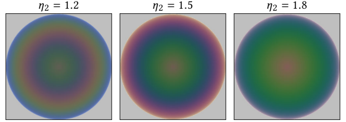
Fig. 10. The Airy reflectance term is directly visualized on spheres with three values of \eta_2 (one per column); other material parameters are held fixed to \mathcal{D}_{\text{inc}} = 1600\text{nm} , \eta_3 = 1.1 , and \kappa_3 = 1.5 . More color fringes are obtained with smaller values of \eta_2 .
