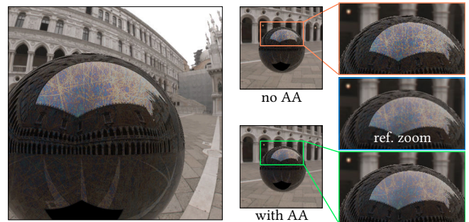
Fig. 15. A highly-detailed texture is mapped to a sphere to produce spatial variations of the film thickness, here applied on a dielectric base layer ( \alpha = 0.01 , \eta_2 = 1.68 , \eta_3 = 2.0 , \mathcal{D}_{inc} \in [0..1470]\text{nm} ). When the sphere is moved away from the camera (middle column), aliasing due to the Airy reflectance term becomes visible, unless we use our dedicated anti-aliasing (AA) technique. As shown in the zoomed insets, our method gives results close to the reference zoomed image.
