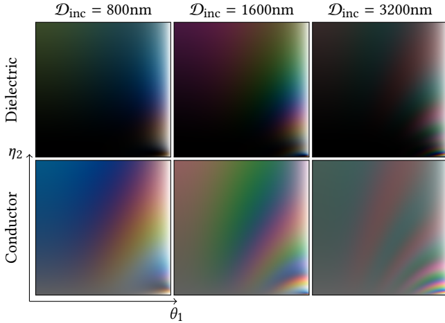
Fig. 9. We show 2D slices of the Airy reflectance term for a base material of index \eta_3 = 1.1 , with either \kappa_3 = 0 (top row) or \kappa_3 = 1.5 (bottom row). In each slice, the horizontal axis maps to \theta_1 , while the vertical axis maps to \eta_2 \in [1..2] . Airy reflectance is highly sensitive to variations of \mathcal{D}_{\text{inc}} at normal incidence.
