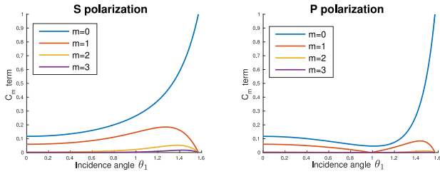
Fig. 22. The C_m terms are visualized for both polarizations (S for perpendicular, P for parallel), as a function of the incidence angle \theta_1 , for a material defined by \eta_2 = 1.5 , \eta_3 = 1.2 and \kappa_3 = 0.5 . All terms but C_0 vanish at \theta_1 = \pi/2 .
