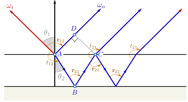
Fig. 4. The complex reflectance coefficient \mathbf{r} from Equation 2 is obtained by summing the reflectance coefficients of light paths of all orders (here we show orders k = \{0, 1, 2\} ), taking into account their interference due to phase shifts. For instance, at order k = 1 , this corresponds to the phase shift between the path going from A to D , and the path going from A to B to C .
