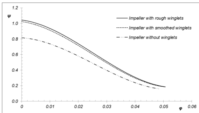
Figure 9. Pressure coefficient over flow coefficient for study 2
