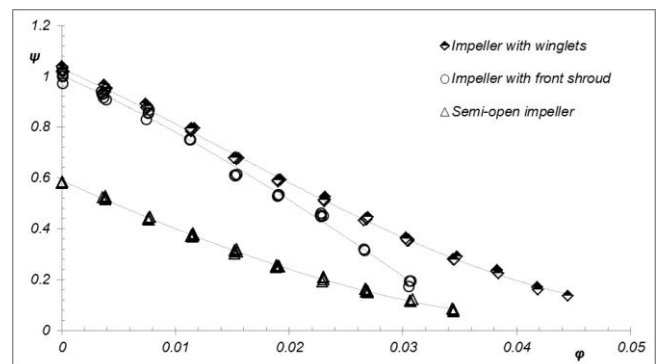
Figure 6. Pressure coefficient over flow coefficient for study 1
