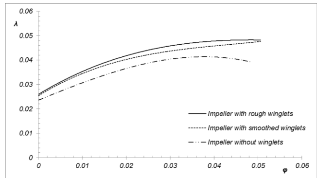
Figure 11. Power coefficient over flow coefficient for study 2
