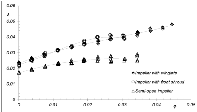
Figure 8. Power coefficient over flow coefficient for study 1
