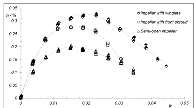
Figure 7. Efficiency over flow coefficient for study 1
