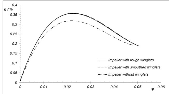
Figure 10. Efficiency over flow coefficient for study 2
