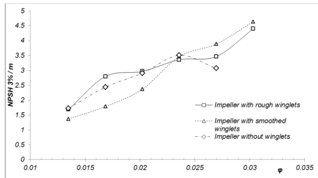
Figure 12. NPSH_{3\%} over flow coefficient for study 2
