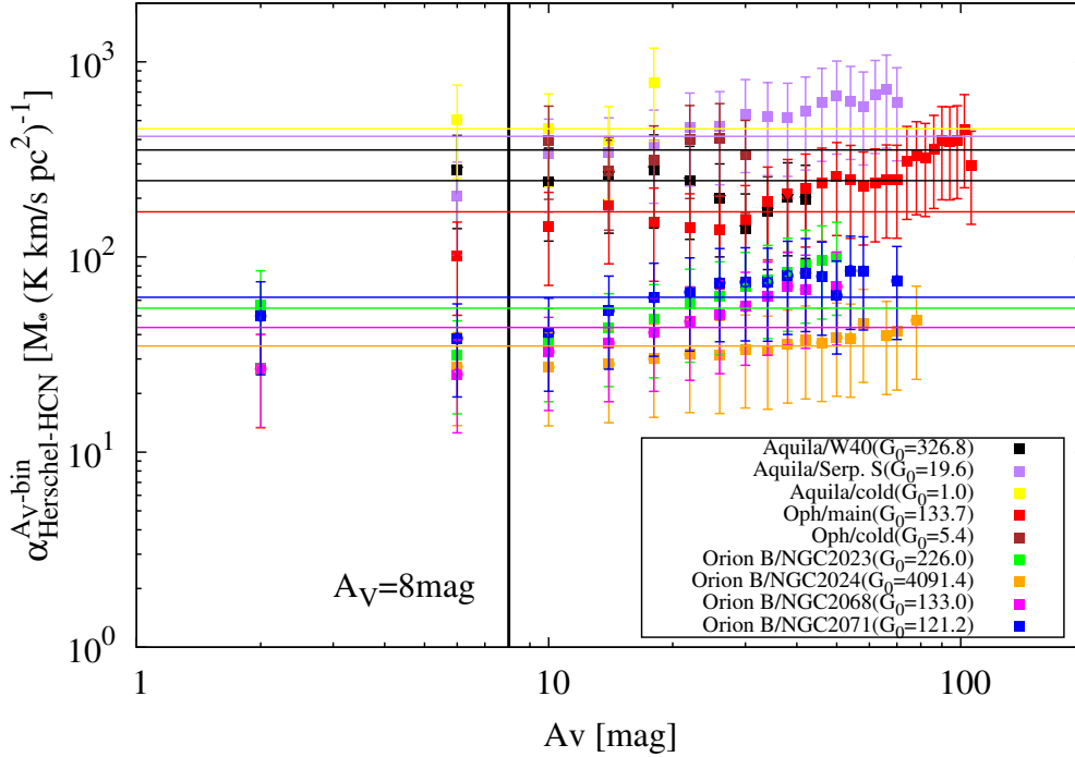
Fig. 6. Empirical conversion factor \alpha_{\text{Herschel-HCN}}^{\text{Av-bin}} \equiv M_{\text{Herschel}}^{\text{Av-bin}} \times L_{\text{HCN}}^{\text{Av-bin}} against column density (expressed in A_V units) for the sub-regions of our sample. M_{\text{Herschel}}^{\text{Av-bin}} and L_{\text{HCN}}^{\text{Av-bin}} represent the mass derived from Herschel column density data and the HCN luminosity for the portion of each sub-region corresponding to a given column density bin. The width of each column density bin is 4 mag in A_V units. The horizontal lines indicate \alpha_{\text{Herschel-HCN}} for the various regions (see Table 6).
