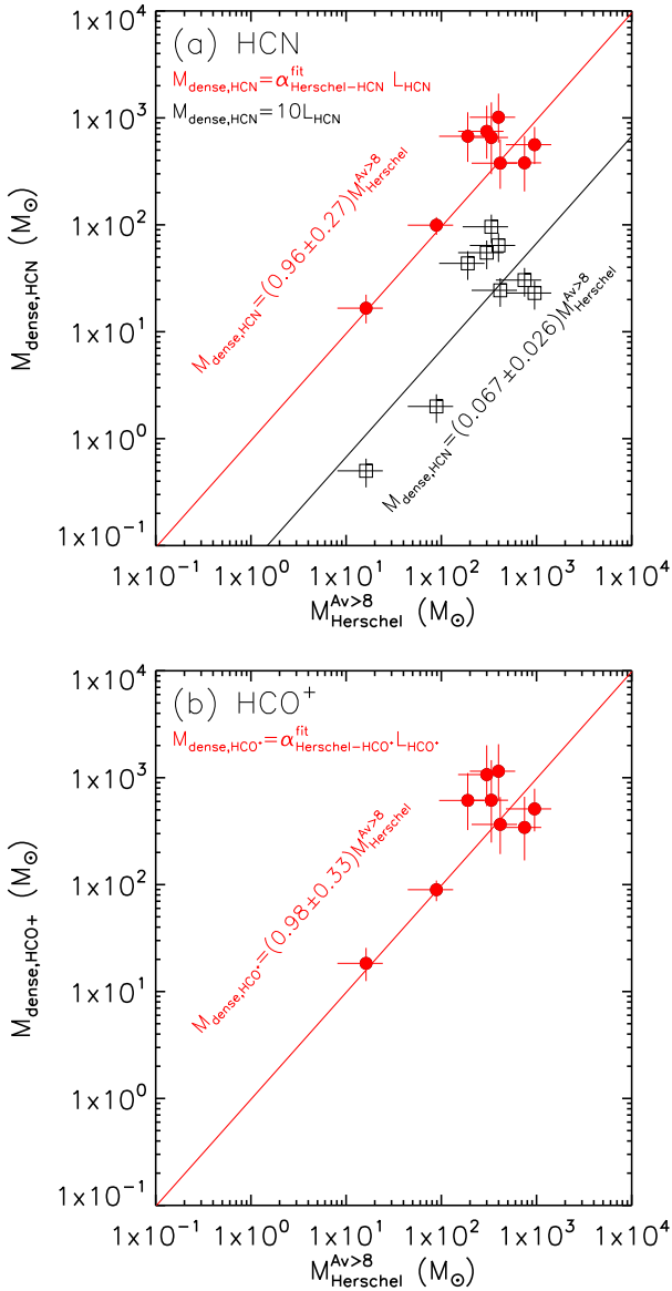
Fig. 5. a) M_{\text{dense,HCN}} against M_{\text{Herschel}}^{\text{Av}>8} and b) M_{\text{dense,HCO}^+} against M_{\text{Herschel}}^{\text{Av}>8} . Red lines correspond to best-fit linear relations to the red data points: M_{\text{dense,HCN}} = (0.96 \pm 0.27) \times M_{\text{Herschel}}^{\text{Av}>8} and M_{\text{dense,HCO}^+} = (0.98 \pm 0.33) \times M_{\text{Herschel}}^{\text{Av}>8} . The red filled circles use M_{\text{dense,mol}} values derived from the relation M_{\text{dense,mol}} = \alpha_{\text{Herschel-mol}}^{\text{fit}} \times L_{\text{mol}} . In panel a , the black open squares use M_{\text{dense,HCN}} values derived from the “extragalactic” relation M_{\text{dense,HCN}} = \alpha_{\text{GS04-HCN}} \times L_{\text{HCN}} , where \alpha_{\text{GS04-HCN}} = 10 M_{\odot} (\text{K km s}^{-1} \text{pc}^2)^{-1} ; the black line corresponds to the best-fit linear relation to the open squares: M_{\text{dense,HCN}} (= \alpha_{\text{GS04-HCN}} L_{\text{HCN}}) = (0.067 \pm 0.026) \times M_{\text{Herschel}}^{\text{Av}>8} .
