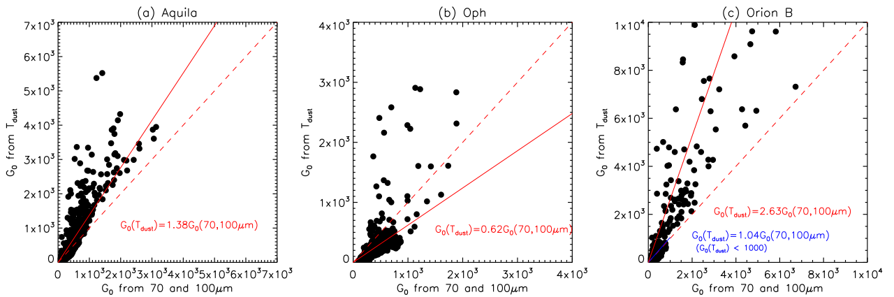
Fig. A.8. Pixel to pixel correlation between the G_0 value estimated from T_{\text{dust}} , G_0(T_{\text{dust}}) , using Eqs. ((11)–(13)) map and G_0 values estimated from Herschel 70 and 100\ \mu\text{m} data, G_0(70, 100\ \mu\text{m}) , using Eqs. (9), (10) toward a) Aquila; b) Ophiuchus; c) Orion B. The dashed red lines indicate G_0(T_{\text{dust}}) = G_0(70, 100\ \mu\text{m}) . The solid red lines indicate the best-fit results: G_0(T_{\text{dust}}) = (1.38 \pm 0.01) \times G_0(70, 100\ \mu\text{m}) for Aquila, G_0(T_{\text{dust}}) = (0.62 \pm 0.01) \times G_0(70, 100\ \mu\text{m}) for Ophiuchus, and G_0(T_{\text{dust}}) = (2.63 \pm 0.09) \times G_0(70, 100\ \mu\text{m}) for Orion B. The blue lines in panel c indicate the best-fit result for pixels with G_0(T_{\text{dust}}) < 1000 : G_0(T_{\text{dust}}) = (1.04 \pm 0.02) \times G_0(70, 100\ \mu\text{m}) .
