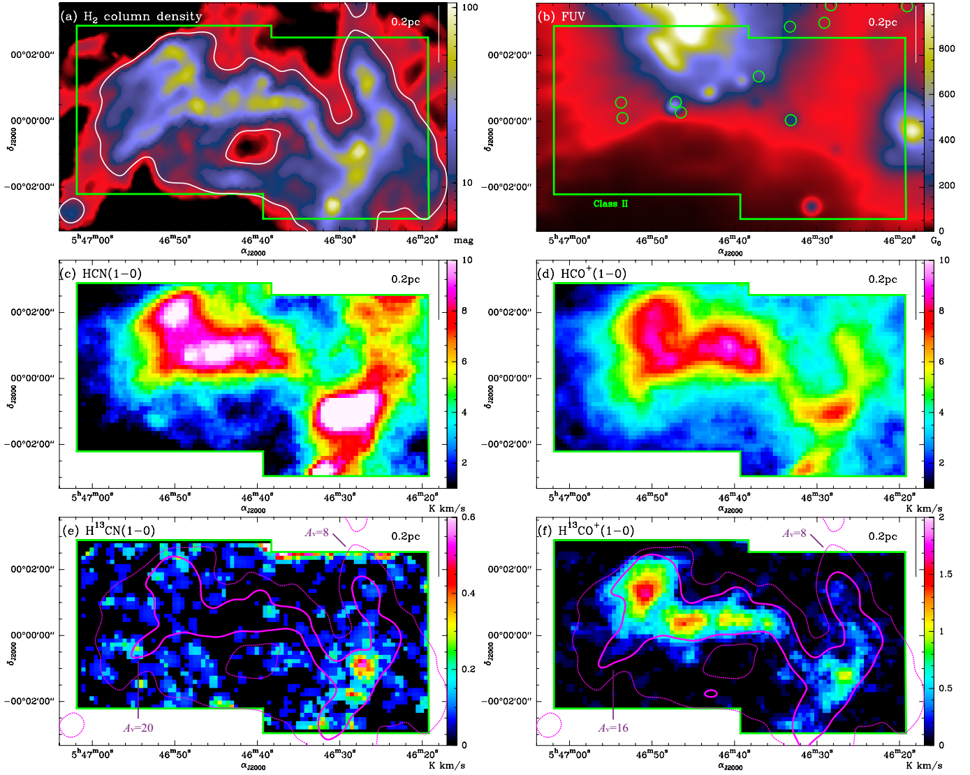
Fig. A.5. Same as Fig. 1, but for NGC 2068 in Orion B. The H 2 column density map of the Orion B region is from HGBS data (Könyves et al., in prep.; see also Schneider et al. 2013). The angular resolutions of HCN, HCO + , and H 13 CO + , and H 13 CN maps are 30'', 30'', 30'', and 40''. The white contour in panel a and magenta dashed contours in panels e and f indicate the A_V = 8 level derived from the Herschel column density map smoothed to 30'' resolution. In panels e and f , the magenta solid contour indicates the rough A_V column density level above which significant line emission is detected, i.e., A_V = 20 for H 13 CN (1-0) and A_V = 16 for H 13 CO + (1-0).
