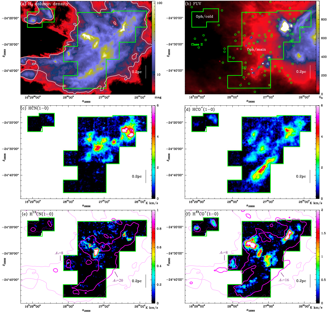
Fig. A.2. Same as Fig. 1, but for Ophiuchus. The \text{H}_2 column density map of the Ophiuchus region is from HGBS data (Ladjetate et al., in prep.). The angular resolutions of HCN, \text{HCO}^+ , and \text{H}^{13}\text{CO}^+ , and \text{H}^{13}\text{CN} maps are 50'' , 50'' , 50'' , and 60'' . The white contour in panel a and magenta dotted contours in panels e and f indicate the A_V = 8 level derived from the Herschel column density map smoothed to 50'' resolution. In panels e and f , the magenta solid contour indicates the rough A_V column density level above which significant line emission is detected, i.e., A_V = 20 for \text{H}^{13}\text{CN} (1–0) and A_V = 16 for \text{H}^{13}\text{CO}^+ (1–0).
