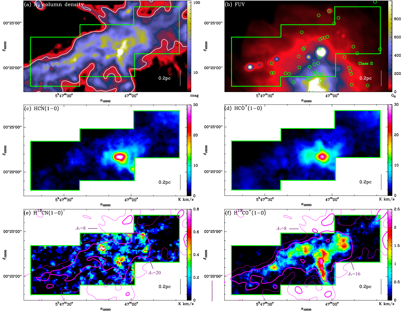
Fig. A.6. Same as Fig. 1, but for NGC 2071 in Orion B. The \text{H}_2 column density map of the Orion B region is from HGBS data (Könyves et al., in prep.; see also Schneider et al. 2013). The angular resolutions of HCN, HCO + , and H 13 CO + , and H 13 CN maps are 30'', 30'', 30'', and 40''. The white contour in panel a and magenta dashed contours in panels e and f indicate the A_V = 8 level derived from the Herschel column density map smoothed to 30'' resolution. In panels e and f , the magenta solid contour indicates the rough A_V column density level above which significant line emission is detected, i.e., A_V = 20 for H 13 CN(1-0) and A_V = 16 for H 13 CO + (1-0).
