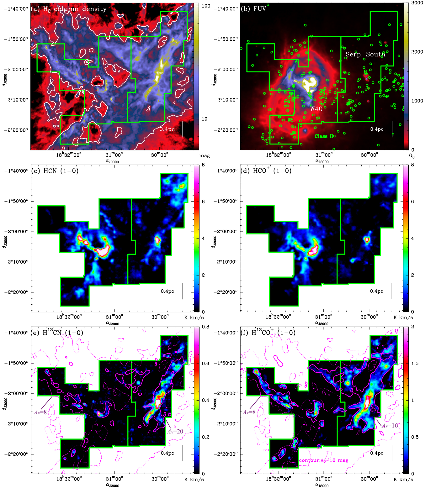
Fig. 1. a ) Column density map of the Aquila region derived from Herschel Gould Belt survey (HGBS) data (André et al. 2010; Könyves et al. 2015) at an angular resolution of 18.2'' and in units of A_V . b ) FUV field strength map derived from HGBS 70\ \mu\text{m} and 100\ \mu\text{m} data smoothed to an angular resolution of 18.2'' in Habing units, and integrated intensity maps of c ) \text{HCN}(1-0) ; d ) \text{HCO}^+(1-0) ; e ) \text{H}^{13}\text{CN}(1-0) ; f ) \text{H}^{13}\text{CO}^+(1-0) in units of \text{K km s}^{-1} ( T_{\text{MB}} ). The angular resolutions of the \text{HCN} , \text{HCO}^+ , \text{H}^{13}\text{CN} , and \text{H}^{13}\text{CO}^+ maps are 40'' , 40'' , 40'' , and 50'' , respectively. In each panel, a green polygon outlines the field observed in molecular lines. The \text{HCN} and \text{H}^{13}\text{CN} integrated intensity includes all components of the hyperfine structure (HFS). The white contour in panel a and the magenta dotted contours in panels e and f show the A_V = 8 level obtained after smoothing the Herschel column density map to 40'' resolution. In panel b , green open circles indicate the positions of the Class II objects identified by Dunham et al. (2015). In panels e and f , the magenta solid contour indicates the rough A_V column density level above which significant line emission is detected, i.e., A_V = 20 for \text{H}^{13}\text{CN}(1-0) and A_V = 16 for \text{H}^{13}\text{CO}^+(1-0) .
