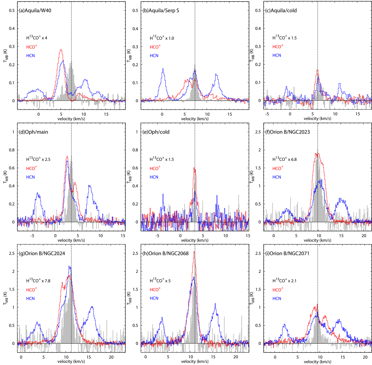
Fig. 3. Comparison of the HCN, HCO + , and H 13 CO + (1–0) spectra averaged over the observed area in a ) Aquila/W40; b ) Aquila/Serp–South; c ) Aquila/cold; d ) Oph/main; e ) Oph/cold; f ) Orion B/NGC 2023; g ) Orion B/NGC 2024; h ) Orion B/NGC 2068; and i ) Orion B/NGC 2071. In each panel, blue, red, and gray lines show the mean HCN, HCO + , and H 13 CO + (1–0) spectra in the corresponding subregion; the vertical dashed line marks the peak velocity of the H 13 CO + (1–0) line.
