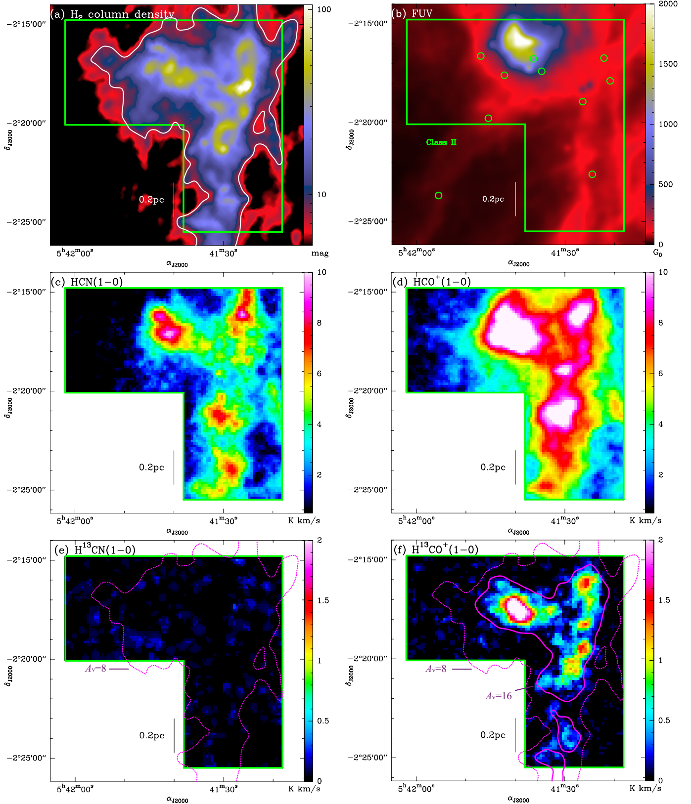
Fig. A.3. Same as Fig. 1, but for NGC 2023 in Orion B. The \text{H}_2 column density map of the Orion B region is from HGBS data (Könyves et al., in prep.; see also Schneider et al. 2013). The angular resolutions of HCN, \text{HCO}^+ , and \text{H}^{13}\text{CO}^+ , and \text{H}^{13}\text{CN} maps are 30'' , 30'' , 30'' , and 40'' . The white contour in panel a and magenta dotted contours in panels e and f indicate the A_V = 8 level derived from the Herschel column density map smoothed to 30'' resolution. In panel f, the magenta solid contour indicates the rough A_V column density level above which significant \text{H}^{13}\text{CO}^+ (1–0) emission is detected, i.e., A_V = 16 .
