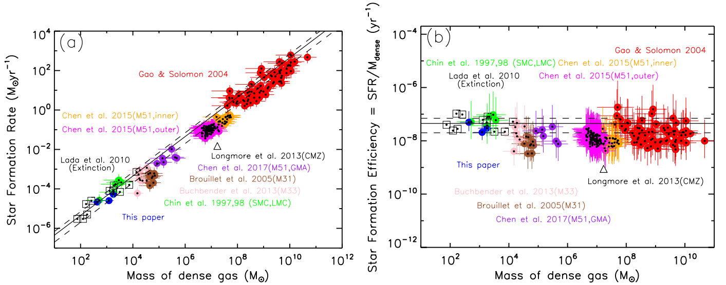
Fig. 7. a) SFR against M_{\text{dense}} and b) SFE against M_{\text{dense}} . Blue filled squares indicate the SFR-M_{\text{dense}} ( =M_{\text{Herschel}}^{A_V > 8} ) and SFE(=SFR/M_{\text{dense}})-M_{\text{dense}} relations for the regions observed in this paper. Black open circles indicate the relation between SFR and M_{\text{dense}} in nearby star-forming clouds (Lada et al. 2010). Red filled circles indicate the SFR-M_{\text{dense}} and SFE-M_{\text{dense}} relations obtained for external galaxies (Gao & Solomon 2004b), assuming M_{\text{dense}} = \alpha_{\text{HCN}} \times L_{\text{HCN}} with the corrected \alpha_{\text{HCN}} values from our Eq. (17). Green, brown, pink, purple, magenta, and orange filled circles indicate the SFR-M_{\text{dense}} and SFE-M_{\text{dense}} relations in the SMC, LMC, M31, M33, and M51 galaxies (Chin et al. 1997, 1998; Brouillet et al. 2005; Buchbender et al. 2013; Chen et al. 2015, 2017) using our relation of Eq. (17). The uncertainties in the extragalactic SFR values are a factor of \sim 2 (cf. Bell 2003). The black triangle indicates the position of the central molecular zone (CMZ: |l| < 1 deg, |b| < 0.5 deg) in each plot, where SFR and M_{\text{dense}} were estimated from the number count of massive YSOs and Herschel column density, respectively (Longmore et al. 2013). In both panels, the black solid line and black dashed lines display the simple empirical relation expected from the “microphysics” of prestellar core formation within filaments described in Sect. 4.3 (see also André et al. 2014; Könyves et al. 2015): SFR = (4.5 \pm 2.5) \times 10^{-8} M_{\odot} \text{yr}^{-1} \times (M_{\text{dense}}/M_{\odot}) , i.e., SFE = (4.5 \pm 2.5) \times 10^{-8} \text{yr}^{-1} .
