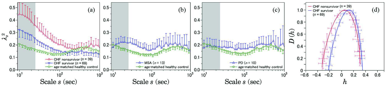
Fig. 6. Scale dependence of the non-Gaussianity index \lambda_s^2 and Multifractal spectrum D(h) of daytime HRV (12:00-18:00). The result for: (a) congestive heart failure (CHF) patients, both for survivors ( n = 69 ) and non-survivors ( n = 39 ) within the follow-up period of 33 \pm 7 months; (b) multiple system atrophy (MSA); and (c) Parkinson disease (PD) patients. Age-matched controls were selected from a database of healthy subjects. Error bars indicate 95%-confidence intervals of the group means. The gray shaded range corresponds to low-frequency band ( s < 25 \text{ sec} ). Marked increases in \lambda_s^2 in the gray shaded scales are observed only in CHF patients, particularly non-survivors (a). D(h) are estimated in the range of 10–200 sec using p -exponent and p -leader based multifractal analysis with p = 1 (see [8] for details). These figures are modified versions from [11].
