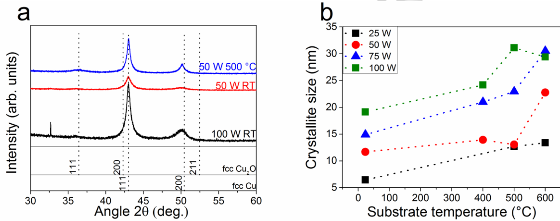
Figure 4: (a) XRD patterns recorded on nc-Cu/C films deposited for 3 deposition conditions ( P_{Cu}=50 W at room temperature and 500 °C, P_{Cu}=100 W). (b) Evolution of the Cu crystallite size for different values of P_{Cu} , deduced from the (111) peak, as a function of the deposition temperature.
