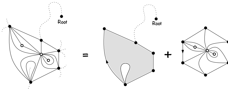
FIGURE 2. Isolating one site-island in a site-percolated triangulation. In the center, we have depicted in gray the face cut in the cluster \dot{\mathfrak{C}} , while on the right we have depicted the site-island corresponding to this face (it is obtained by cutting along both sides of the edges of \dot{\mathfrak{C}} ). Note that some vertices of \dot{\mathfrak{C}} are duplicated, and that this leads to a simple boundary for the site island.
