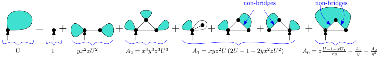
FIGURE 9. Recursive decomposition of triangulations in \mathcal{T} giving (36). Among the triangulations such that the root edge is not a bridge, we distinguish different cases according to the number of bridges created when deleting the root edge: we denote A_0, A_1, A_2 respectively the contribution of the triangulations such that 0, 1 or 2 bridges are created.
