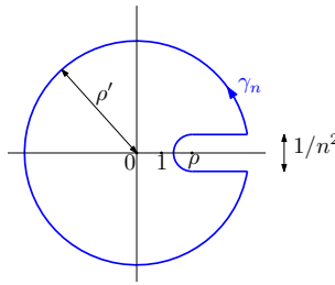
FIGURE 7. The Hankel contour used in the residue calculation.
