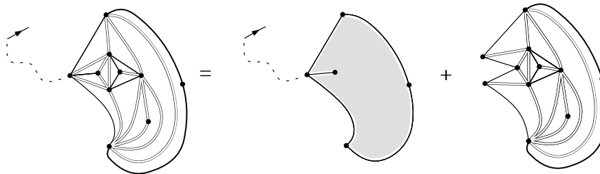
FIGURE 4. Isolating one bond-island in a bond-percolated triangulation. In the center, we have depicted in gray the face cut in the cluster \bar{\mathfrak{C}} , while on the right we have depicted the bond-island corresponding to this face (note that it has a simple boundary).
