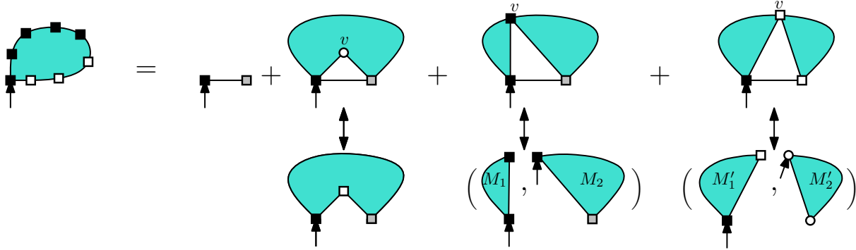
FIGURE 8. Recursive decomposition of maps in \mathcal{R} , by deletion of the root edge. The arrows indicate the root-corners. The outer vertices of maps in \mathcal{R} are indicated by squares colored black if they are active, white if they are inactive, and gray when they could be either.
