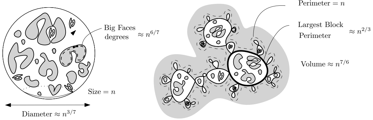
FIGURE 11. Anatomy of a large critical percolation cluster on the (unlikely) event that it has size n (left). On the right, the geometry of a large critical percolation with a boundary of perimeter n .
