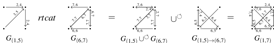
Figure 3: Example of round trip transitive closures concatenation. Labels arr and dep on an edge u \xrightarrow{arr, dep} v (shifted toward the tip) represent respectively arrival(u, v, G(i,j)) and departure(u, v, G(i,j)) .
