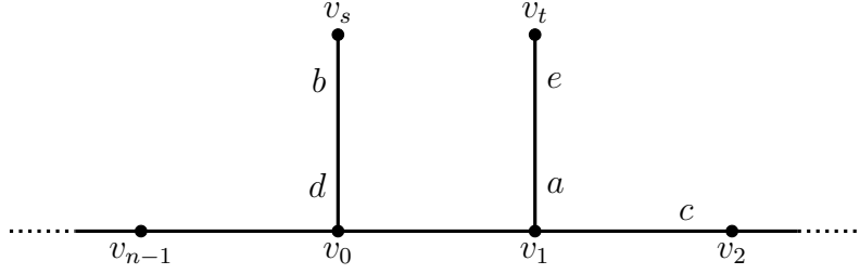
Figure 12: Configuration for the proof of Claim 3.
