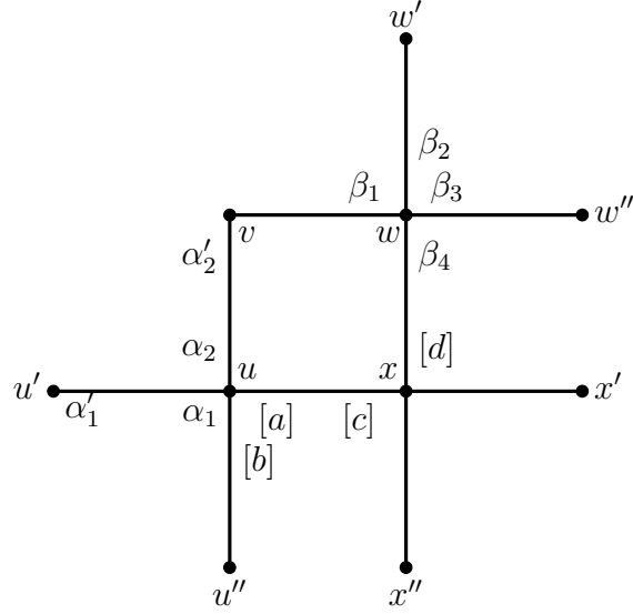
Figure 2: The partially L_0 -list incidence coloured graph H_0 of Lemma 8.
