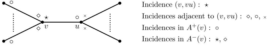
Figure 1: Adjacent incidences.
