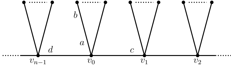
Figure 10: Colouring the external incidences of v_1 ( v_{n-1} = v_2 if n = 3 ), pre-coloured case.
