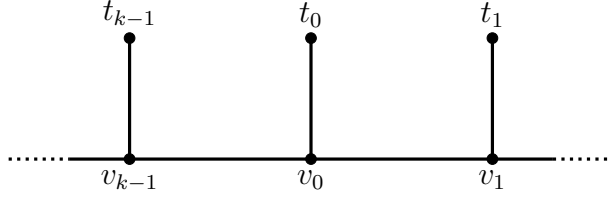
Figure 5: Part of the outer cycle C_G of a Halin graph G (the t_i 's are not necessarily distinct).
