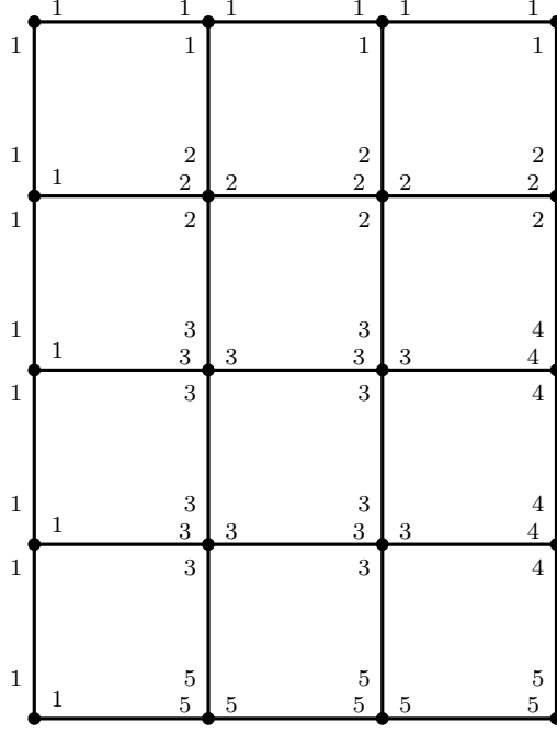
Figure 3: Colouring the incidences of G_{5,4} in five steps (Theorem 9).
