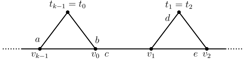
Figure 6: Configuration for the proof of Lemma 12.
